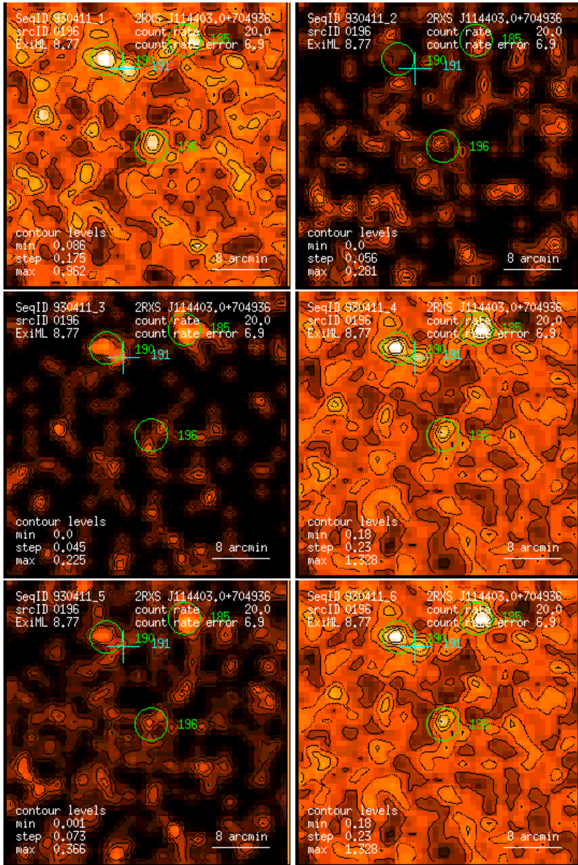
Figure 196: RASS 930411: detection 0196: band rate images, Gaussian filter: (1) PSPC channels 11 – 41, (2) 52 – 90, (3) 91 – 201, (4) 11 – 235, (5) 52 – 201, (6) 11 – 201. Broad band rates in counts/ks. Band rate contour levels in counts/ks/arcmin 2 .
