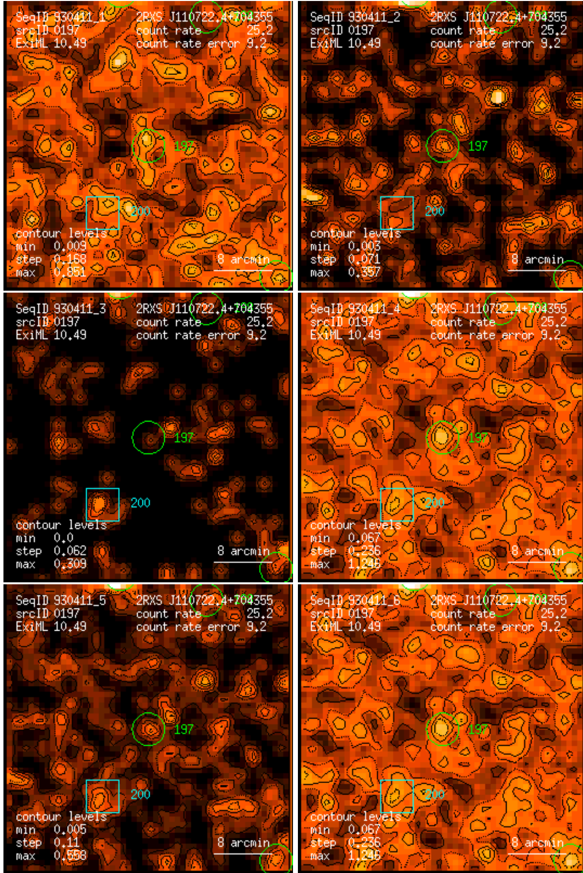
Figure 197: RASS 930411: detection 0197: band rate images, Gaussian filter: (1) PSPC channels 11 – 41, (2) 52 – 90, (3) 91 – 201, (4) 11 – 235, (5) 52 – 201, (6) 11 – 201. Broad band rates in counts/ks. Band rate contour levels in counts/ks/arcmin 2 .
