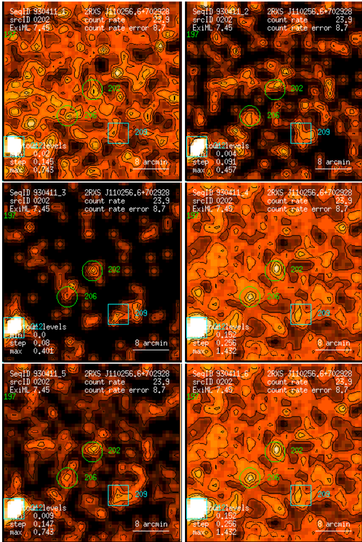
Figure 202: RASS 930411: detection 0202: band rate images, Gaussian filter: (1) PSPC channels 11 – 41, (2) 52 – 90, (3) 91 – 201, (4) 11 – 235, (5) 52 – 201, (6) 11 – 201. Broad band rates in counts/ks. Band rate contour levels in counts/ks/arcmin 2 .
