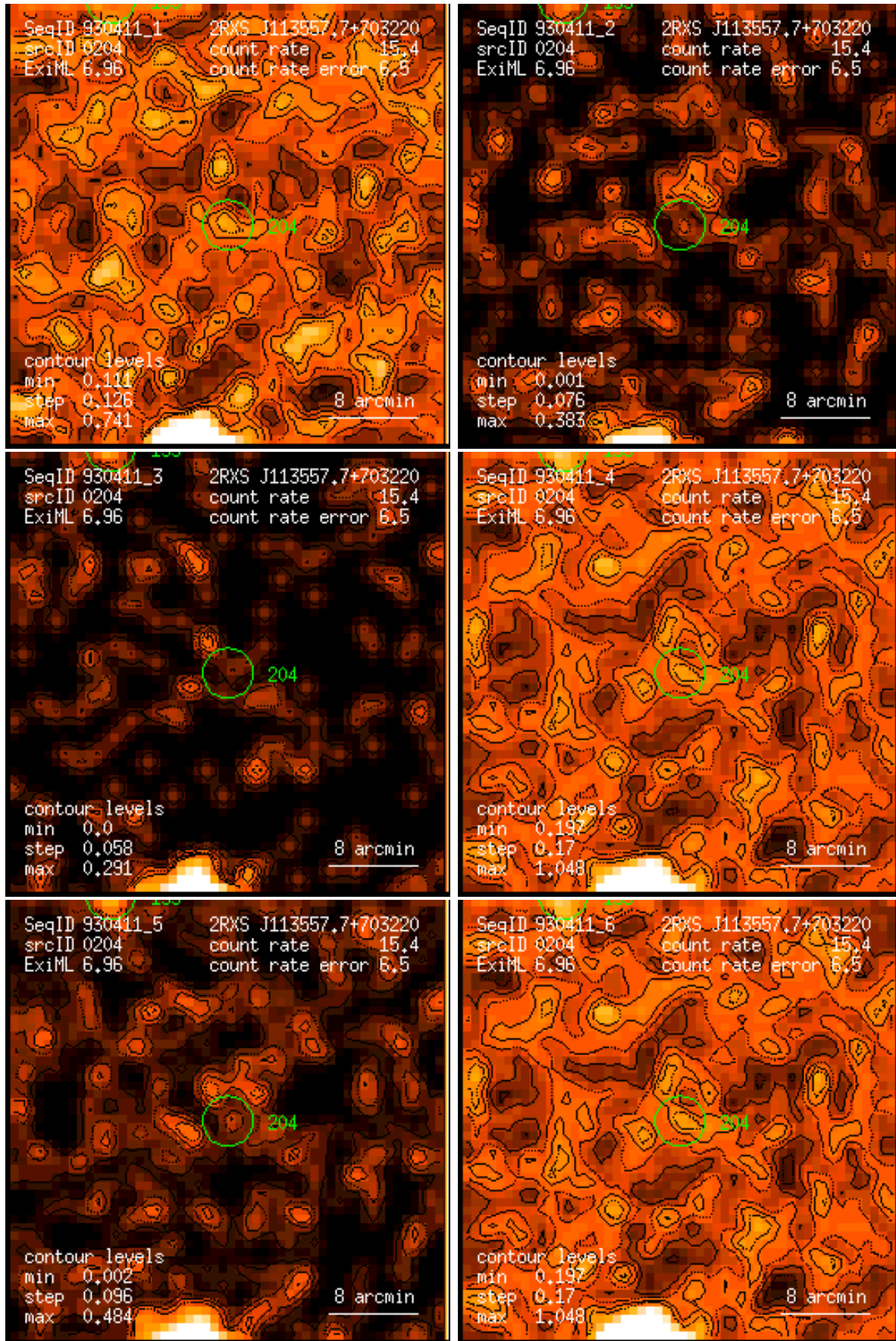
Figure 204: RASS 930411: detection 0204: band rate images, Gaussian filter: (1) PSPC channels 11 – 41, (2) 52 – 90, (3) 91 – 201, (4) 11 – 235, (5) 52 – 201, (6) 11 – 201. Broad band rates in counts/ks. Band rate contour levels in counts/ks/arcmin 2 .
