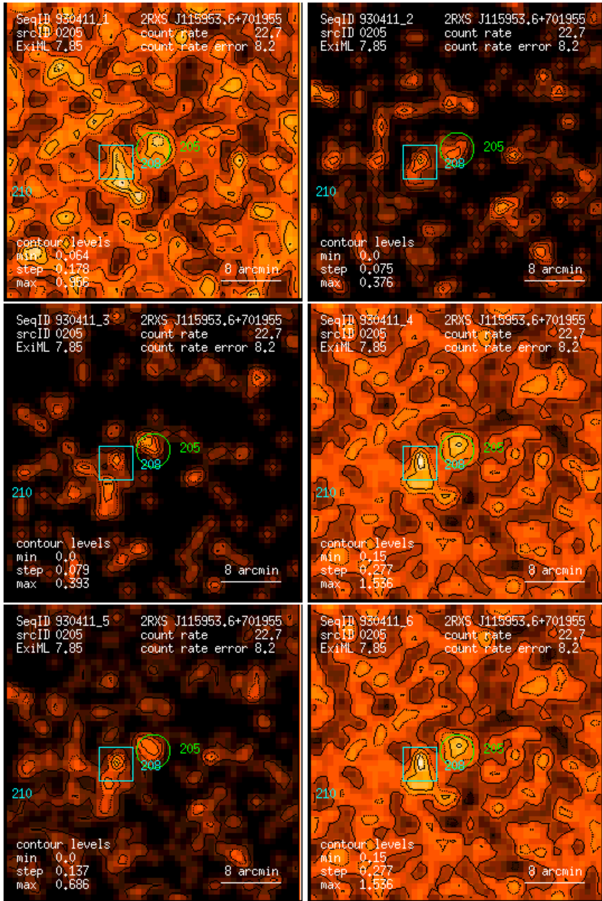
Figure 205: RASS 930411: detection 0205: band rate images, Gaussian filter: (1) PSPC channels 11 – 41, (2) 52 – 90, (3) 91 – 201, (4) 11 – 235, (5) 52 – 201, (6) 11 – 201. Broad band rates in counts/ks. Band rate contour levels in counts/ks/arcmin 2 .
