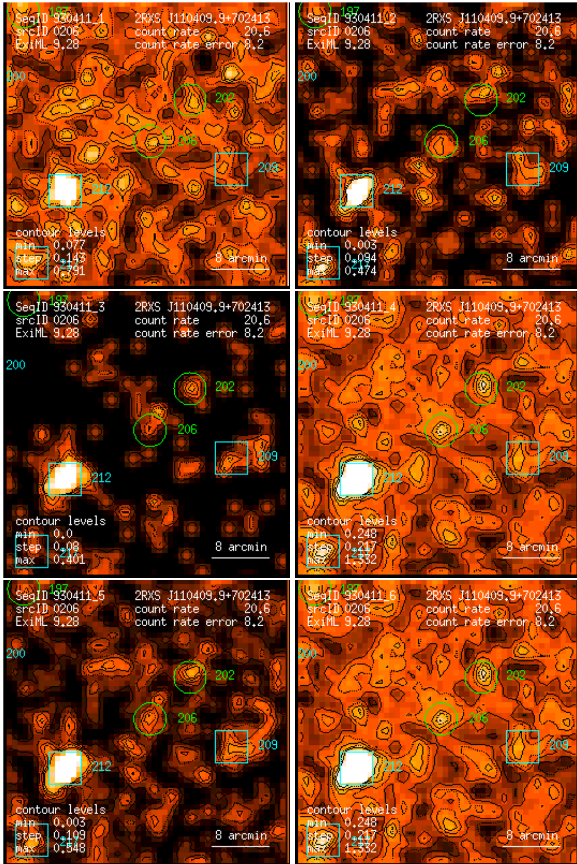
Figure 206: RASS 930411: detection 0206: band rate images, Gaussian filter: (1) PSPC channels 11 – 41, (2) 52 – 90, (3) 91 – 201, (4) 11 – 235, (5) 52 – 201, (6) 11 – 201. Broad band rates in counts/ks. Band rate contour levels in counts/ks/arcmin 2 .
