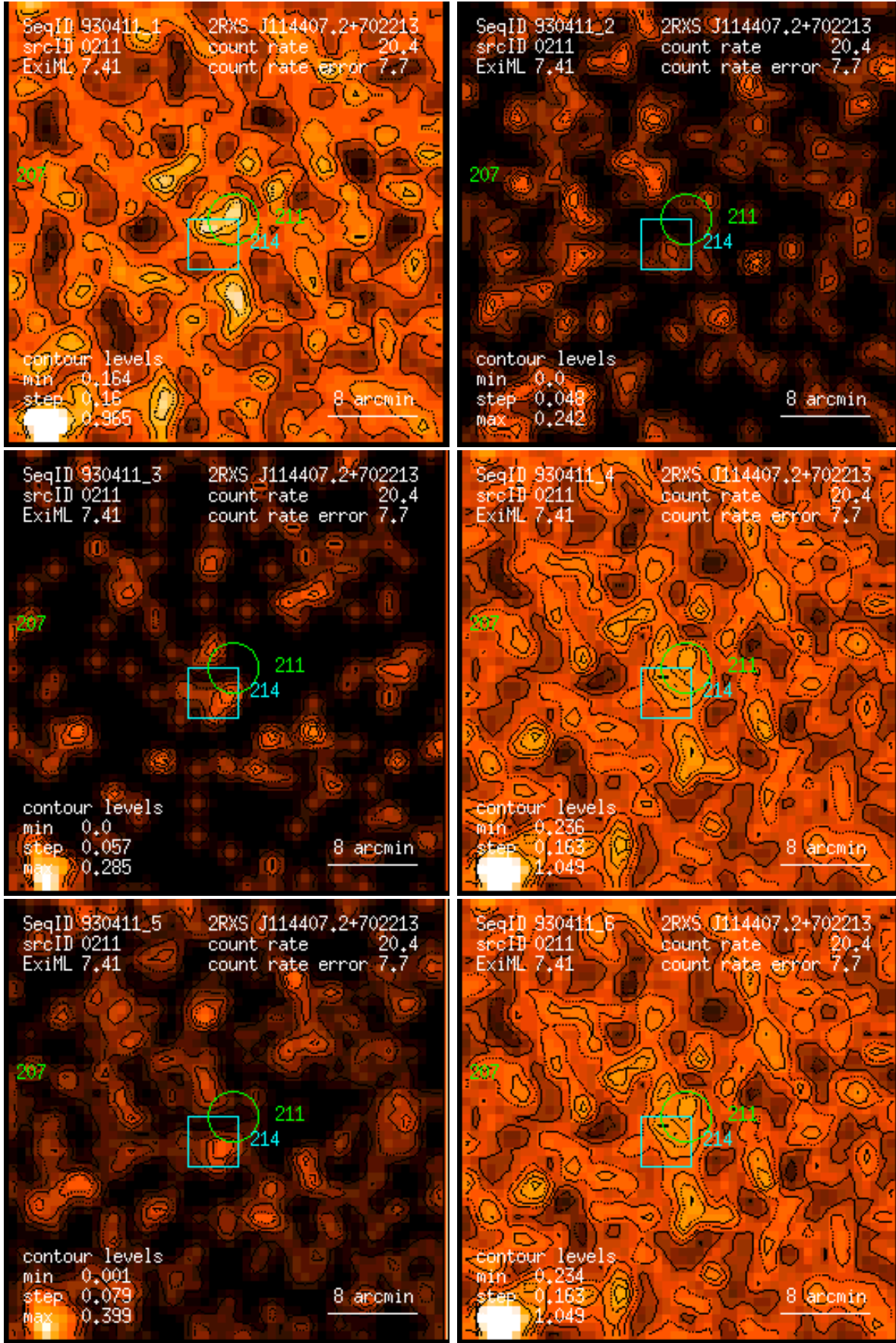
Figure 211: RASS 930411: detection 0211: band rate images, Gaussian filter: (1) PSPC channels 11 – 41, (2) 52 – 90, (3) 91 – 201, (4) 11 – 235, (5) 52 – 201, (6) 11 – 201. Broad band rates in counts/ks. Band rate contour levels in counts/ks/arcmin 2 .
