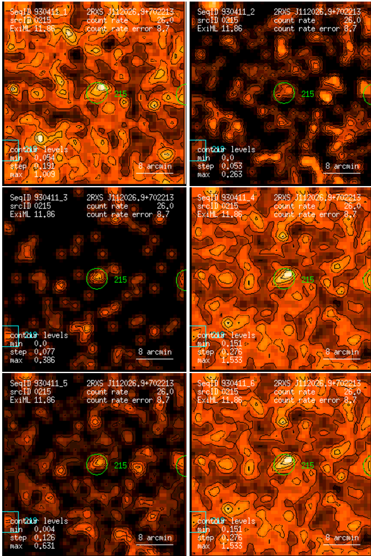
Figure 215: RASS 930411: detection 0215: band rate images, Gaussian filter: (1) PSPC channels 11 – 41, (2) 52 – 90, (3) 91 – 201, (4) 11 – 235, (5) 52 – 201, (6) 11 – 201. Broad band rates in counts/ks. Band rate contour levels in counts/ks/arcmin 2 .
