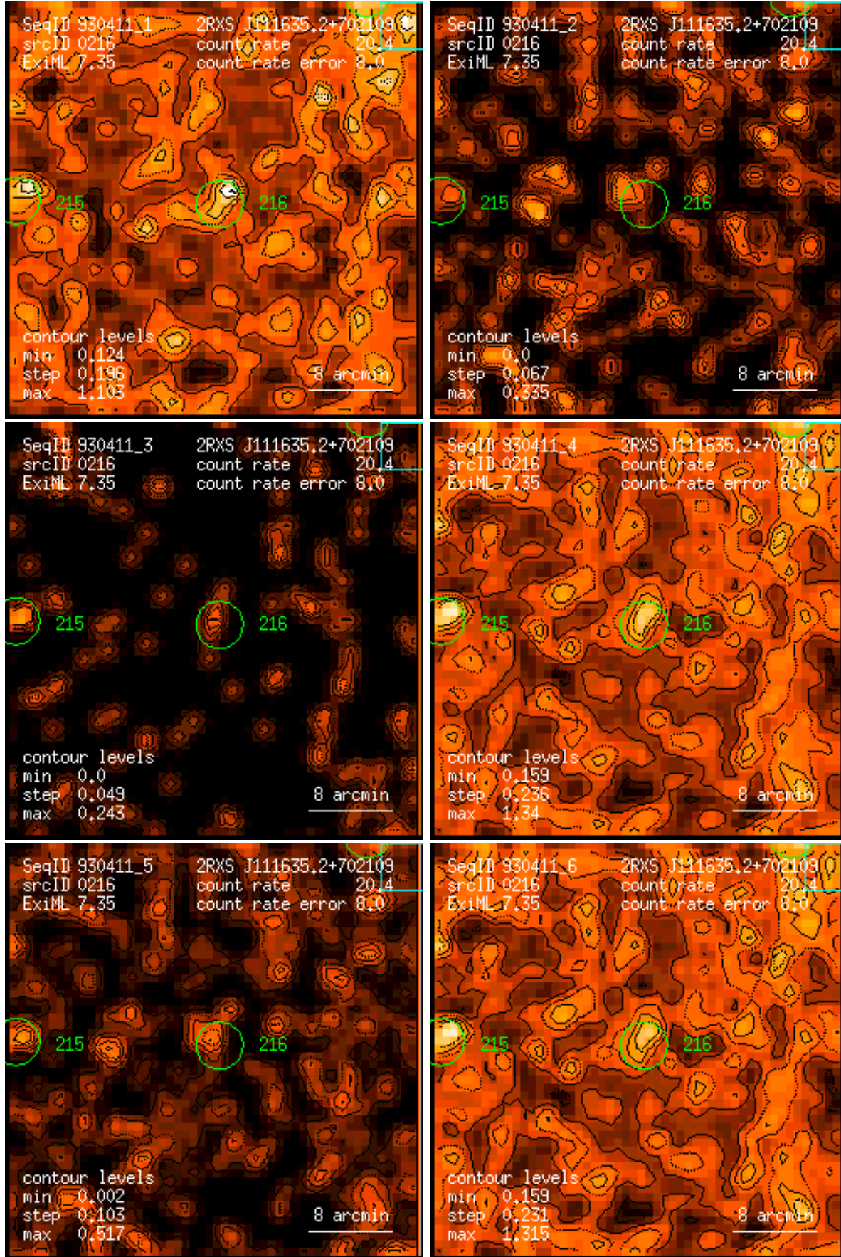
Figure 216: RASS 930411: detection 0216: band rate images, Gaussian filter: (1) PSPC channels 11 – 41, (2) 52 – 90, (3) 91 – 201, (4) 11 – 235, (5) 52 – 201, (6) 11 – 201. Broad band rates in counts/ks. Band rate contour levels in counts/ks/arcmin 2 .
