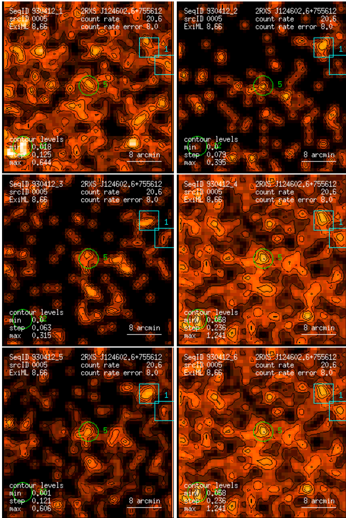
Figure 5: RASS 930412: detection 0005: band rate images, Gaussian filter: (1) PSPC channels 11 – 41, (2) 52 – 90, (3) 91 – 201, (4) 11 – 235, (5) 52 – 201, (6) 11 – 201. Broad band rates in counts/ks. Band rate contour levels in counts/ks/arcmin 2 .
