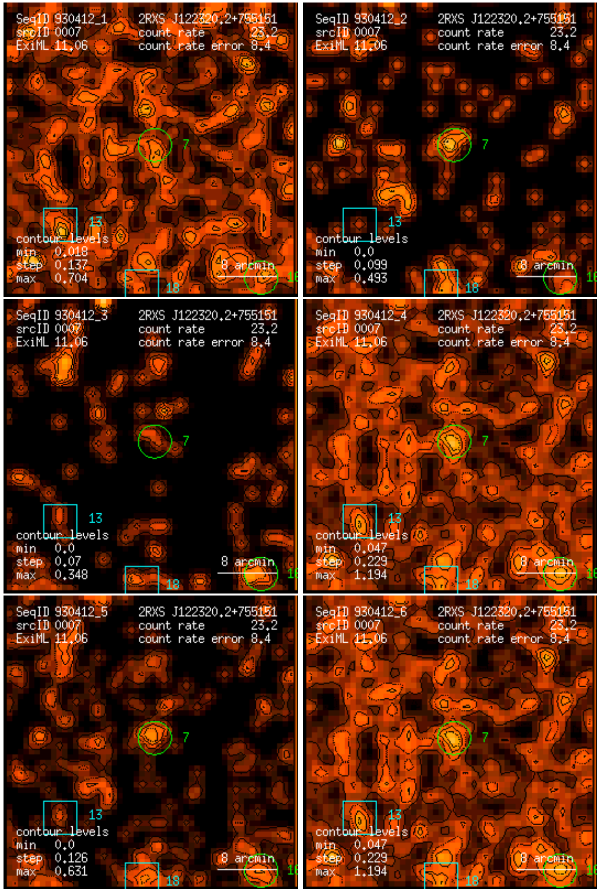
Figure 7: RASS 930412: detection 0007: band rate images, Gaussian filter: (1) PSPC channels 11 – 41, (2) 52 – 90, (3) 91 – 201, (4) 11 – 235, (5) 52 – 201, (6) 11 – 201. Broad band rates in counts/ks. Band rate contour levels in counts/ks/arcmin 2 .
