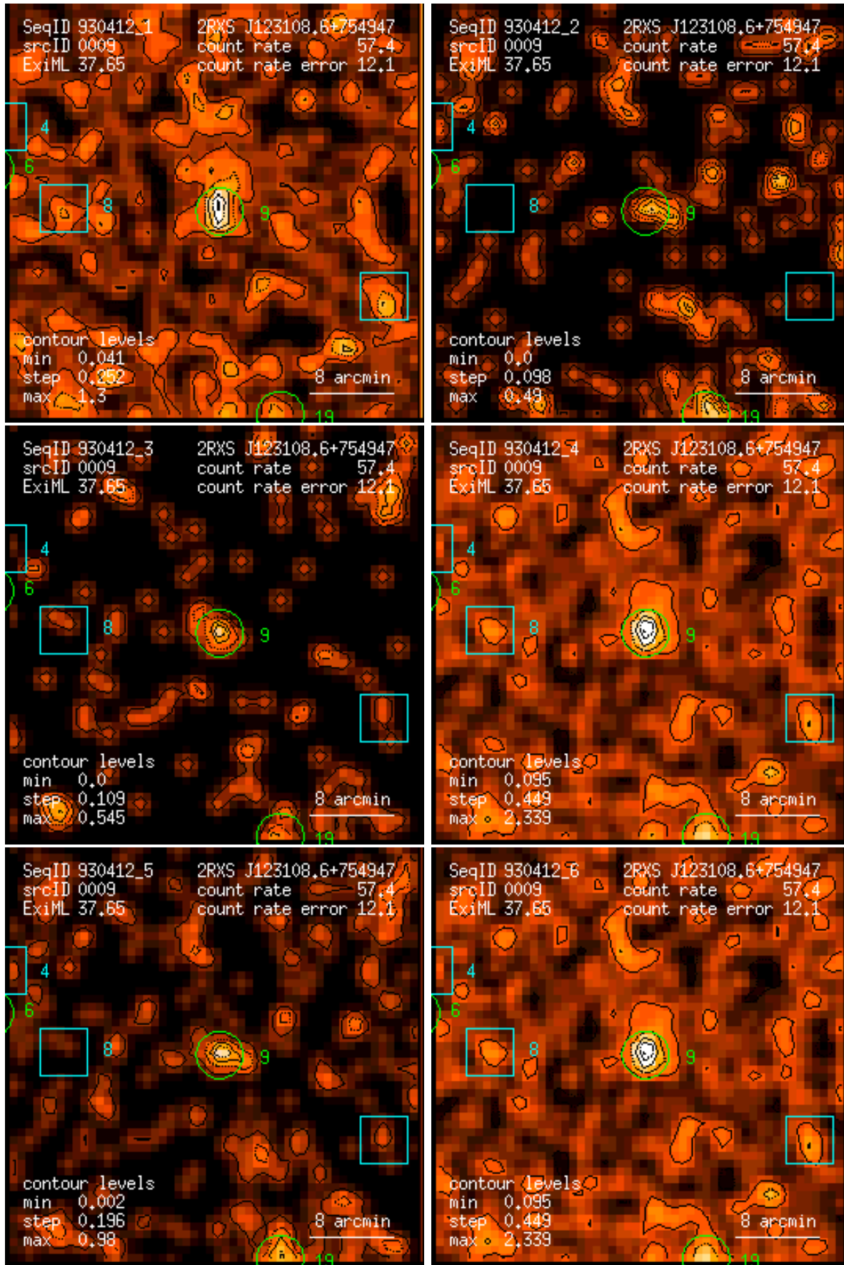
Figure 9: RASS 930412: detection 0009: band rate images, Gaussian filter: (1) PSPC channels 11 – 41, (2) 52 – 90, (3) 91 – 201, (4) 11 – 235, (5) 52 – 201, (6) 11 – 201. Broad band rates in counts/ks. Band rate contour levels in counts/ks/arcmin 2 .
