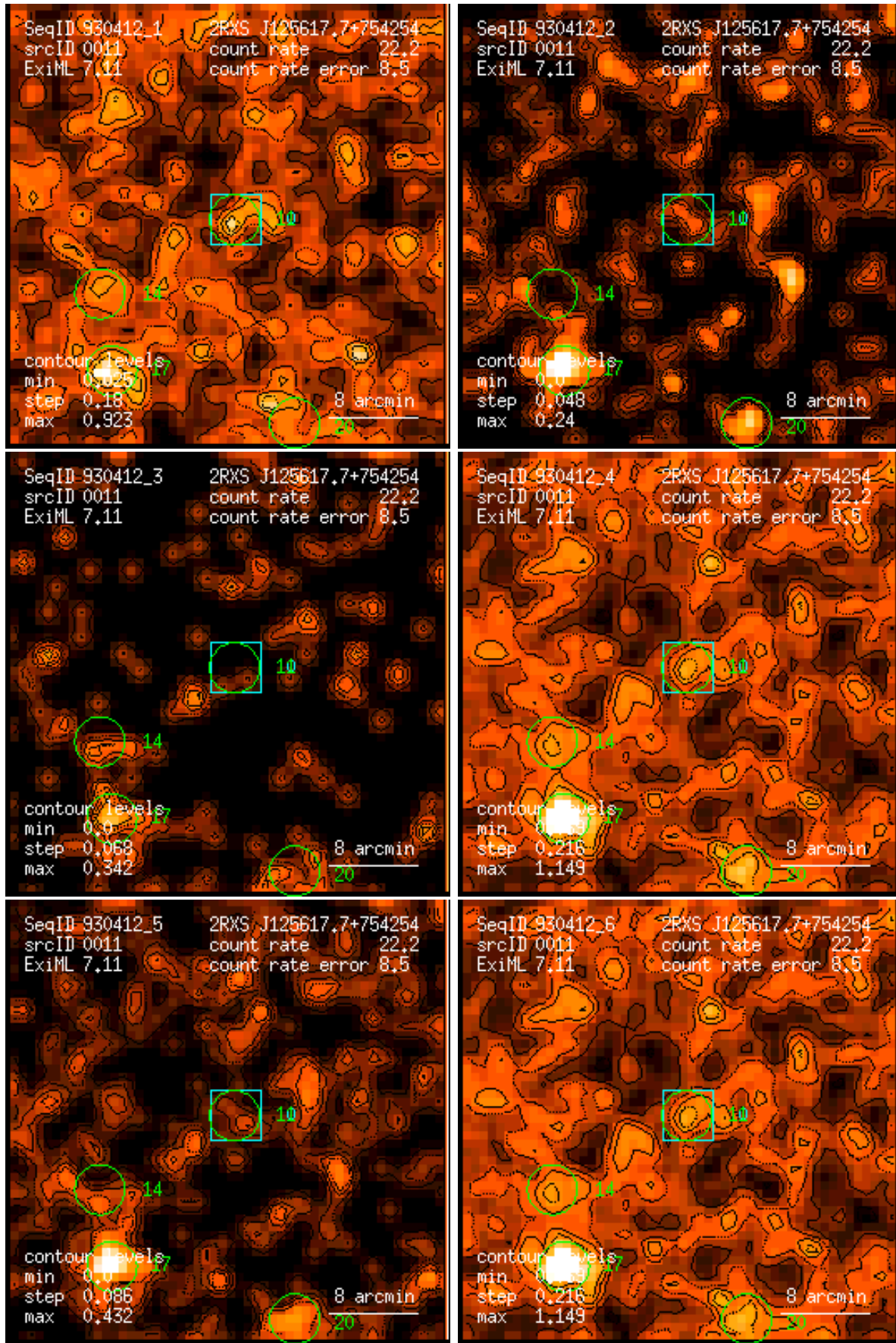
Figure 11: RASS 930412: detection 0011: band rate images, Gaussian filter: (1) PSPC channels 11 – 41, (2) 52 – 90, (3) 91 – 201, (4) 11 – 235, (5) 52 – 201, (6) 11 – 201. Broad band rates in counts/ks. Band rate contour levels in counts/ks/arcmin 2 .
