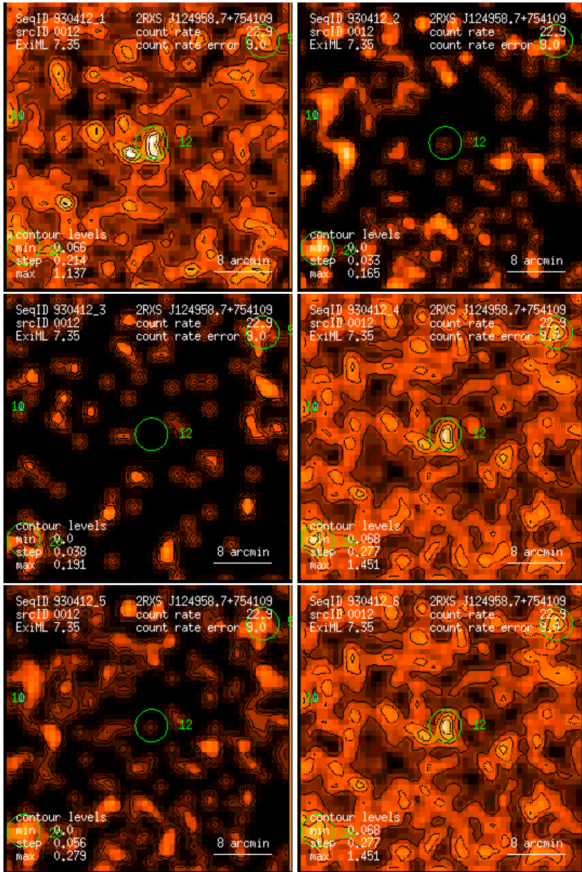
Figure 12: RASS 930412: detection 0012: band rate images, Gaussian filter: (1) PSPC channels 11 – 41, (2) 52 – 90, (3) 91 – 201, (4) 11 – 235, (5) 52 – 201, (6) 11 – 201. Broad band rates in counts/ks. Band rate contour levels in counts/ks/arcmin 2 .
