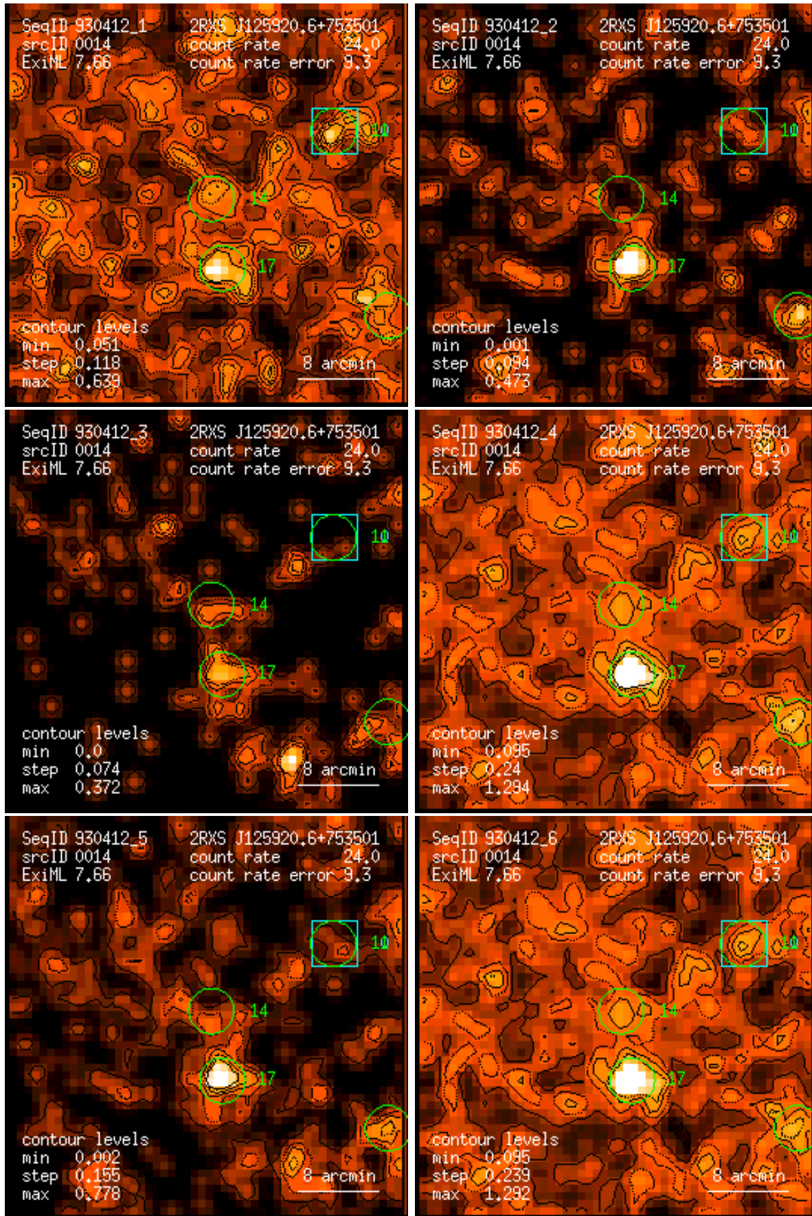
Figure 14: RASS 930412: detection 0014: band rate images, Gaussian filter: (1) PSPC channels 11 – 41, (2) 52 – 90, (3) 91 – 201, (4) 11 – 235, (5) 52 – 201, (6) 11 – 201. Broad band rates in counts/ks. Band rate contour levels in counts/ks/arcmin 2 .
