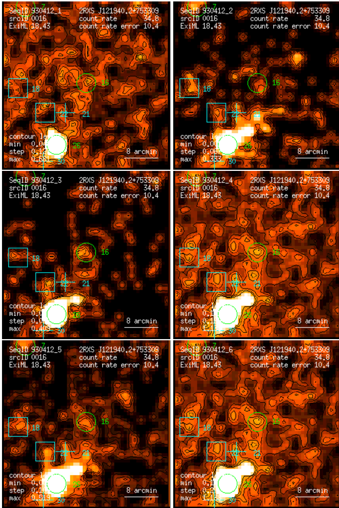
Figure 16: RASS 930412: detection 0016: band rate images, Gaussian filter: (1) PSPC channels 11 – 41, (2) 52 – 90, (3) 91 – 201, (4) 11 – 235, (5) 52 – 201, (6) 11 – 201. Broad band rates in counts/ks. Band rate contour levels in counts/ks/arcmin 2 .
