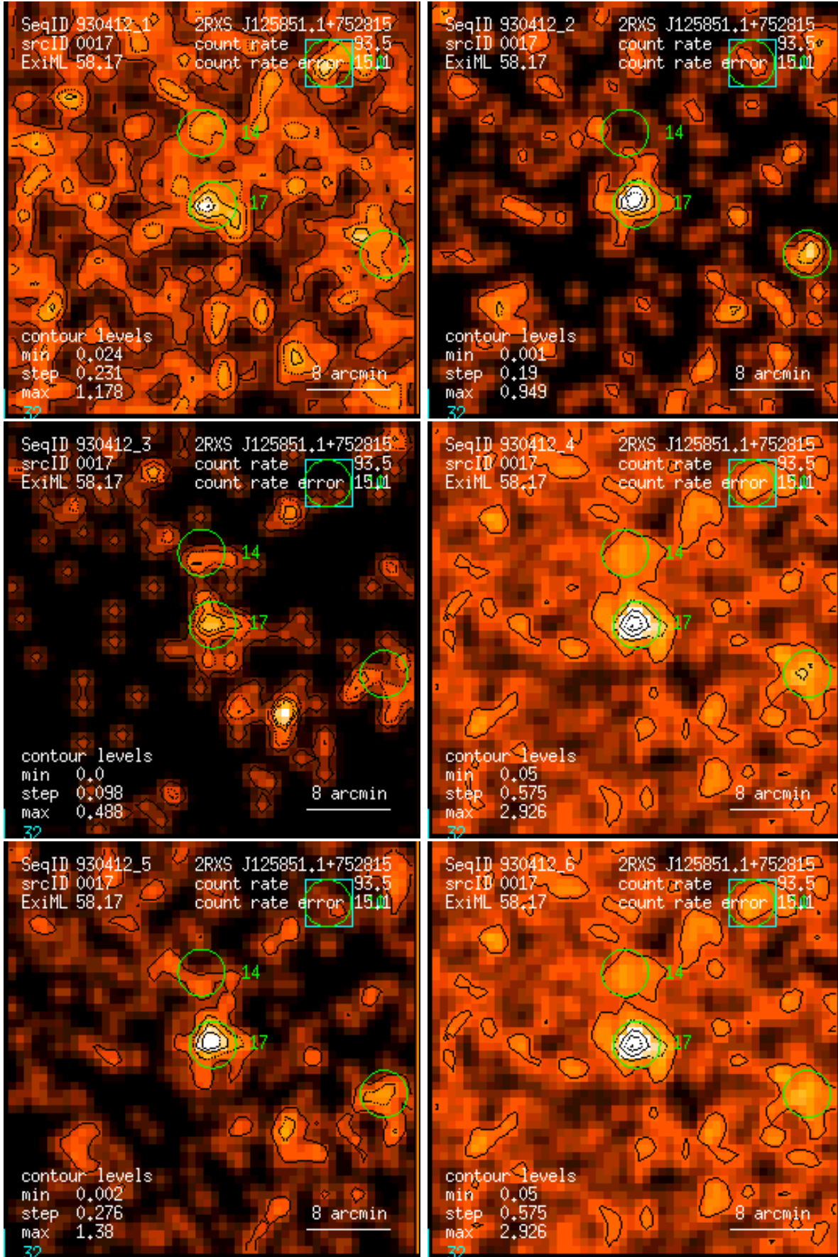
Figure 17: RASS 930412: detection 0017: band rate images, Gaussian filter: (1) PSPC channels 11 – 41, (2) 52 – 90, (3) 91 – 201, (4) 11 – 235, (5) 52 – 201, (6) 11 – 201. Broad band rates in counts/ks. Band rate contour levels in counts/ks/arcmin 2 .
