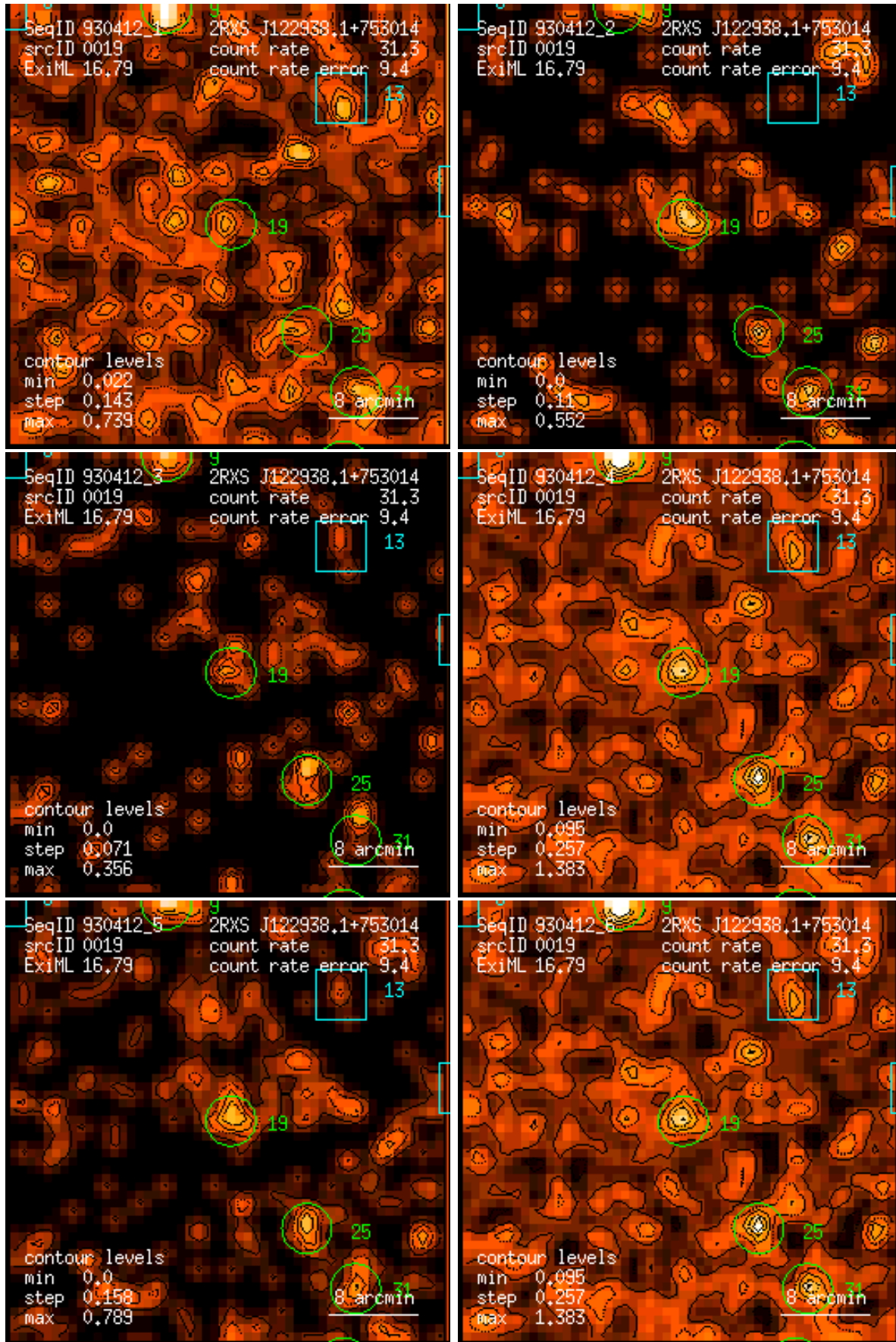
Figure 19: RASS 930412: detection 0019: band rate images, Gaussian filter: (1) PSPC channels 11 – 41, (2) 52 – 90, (3) 91 – 201, (4) 11 – 235, (5) 52 – 201, (6) 11 – 201. Broad band rates in counts/ks. Band rate contour levels in counts/ks/arcmin 2 .
