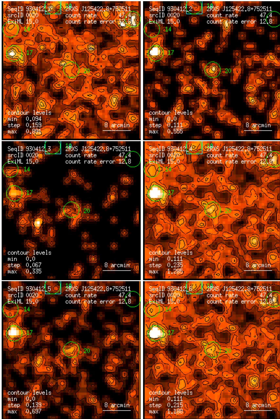
Figure 20: RASS 930412: detection 0020: band rate images, Gaussian filter: (1) PSPC channels 11 – 41, (2) 52 – 90, (3) 91 – 201, (4) 11 – 235, (5) 52 – 201, (6) 11 – 201. Broad band rates in counts/ks. Band rate contour levels in counts/ks/arcmin 2 .
