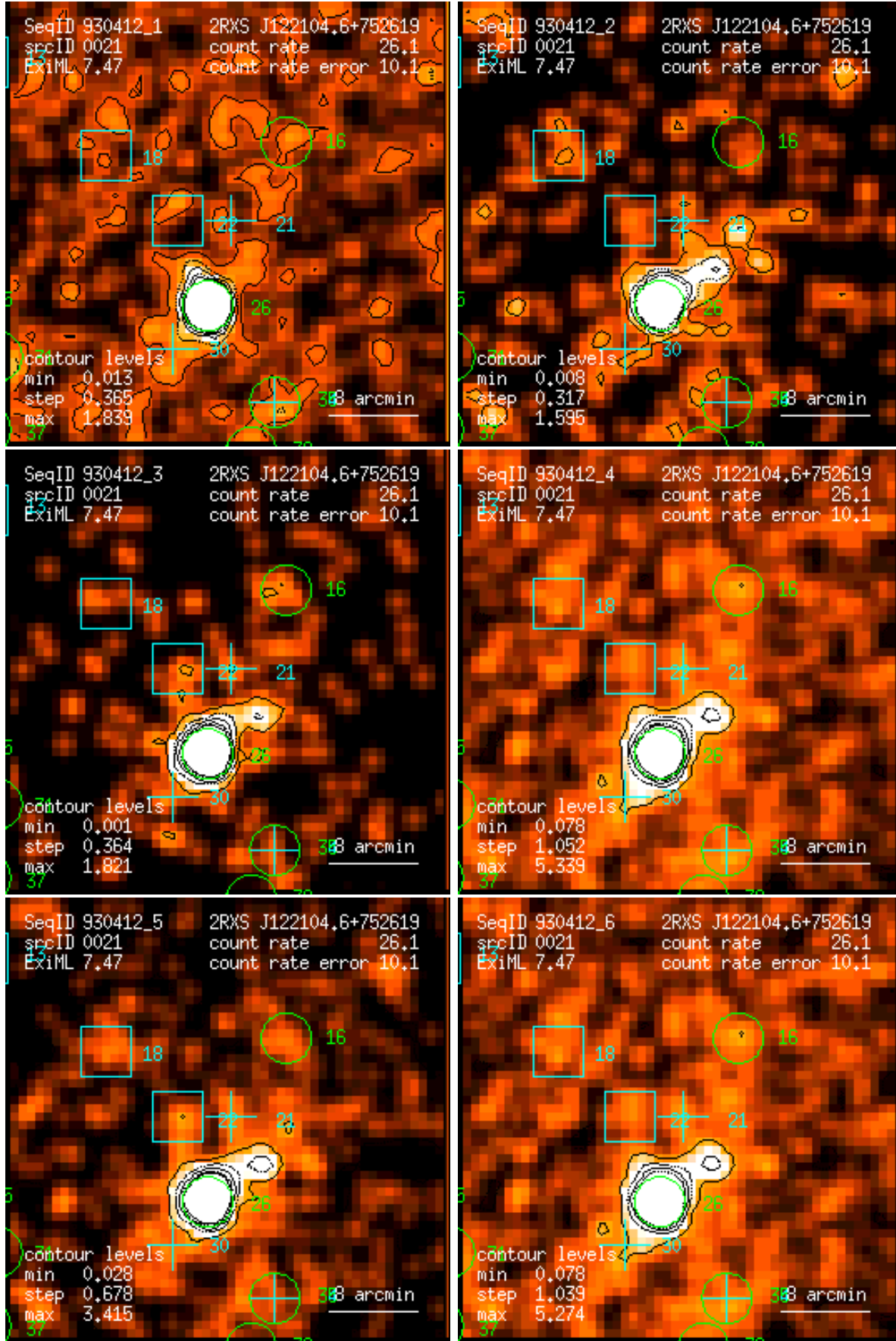
Figure 21: RASS 930412: detection 0021: band rate images, Gaussian filter: (1) PSPC channels 11 – 41, (2) 52 – 90, (3) 91 – 201, (4) 11 – 235, (5) 52 – 201, (6) 11 – 201. Broad band rates in counts/ks. Band rate contour levels in counts/ks/arcmin 2 .
