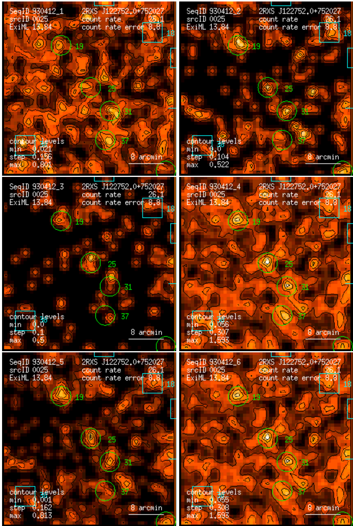
Figure 25: RASS 930412: detection 0025: band rate images, Gaussian filter: (1) PSPC channels 11 – 41, (2) 52 – 90, (3) 91 – 201, (4) 11 – 235, (5) 52 – 201, (6) 11 – 201. Broad band rates in counts/ks. Band rate contour levels in counts/ks/arcmin 2 .
