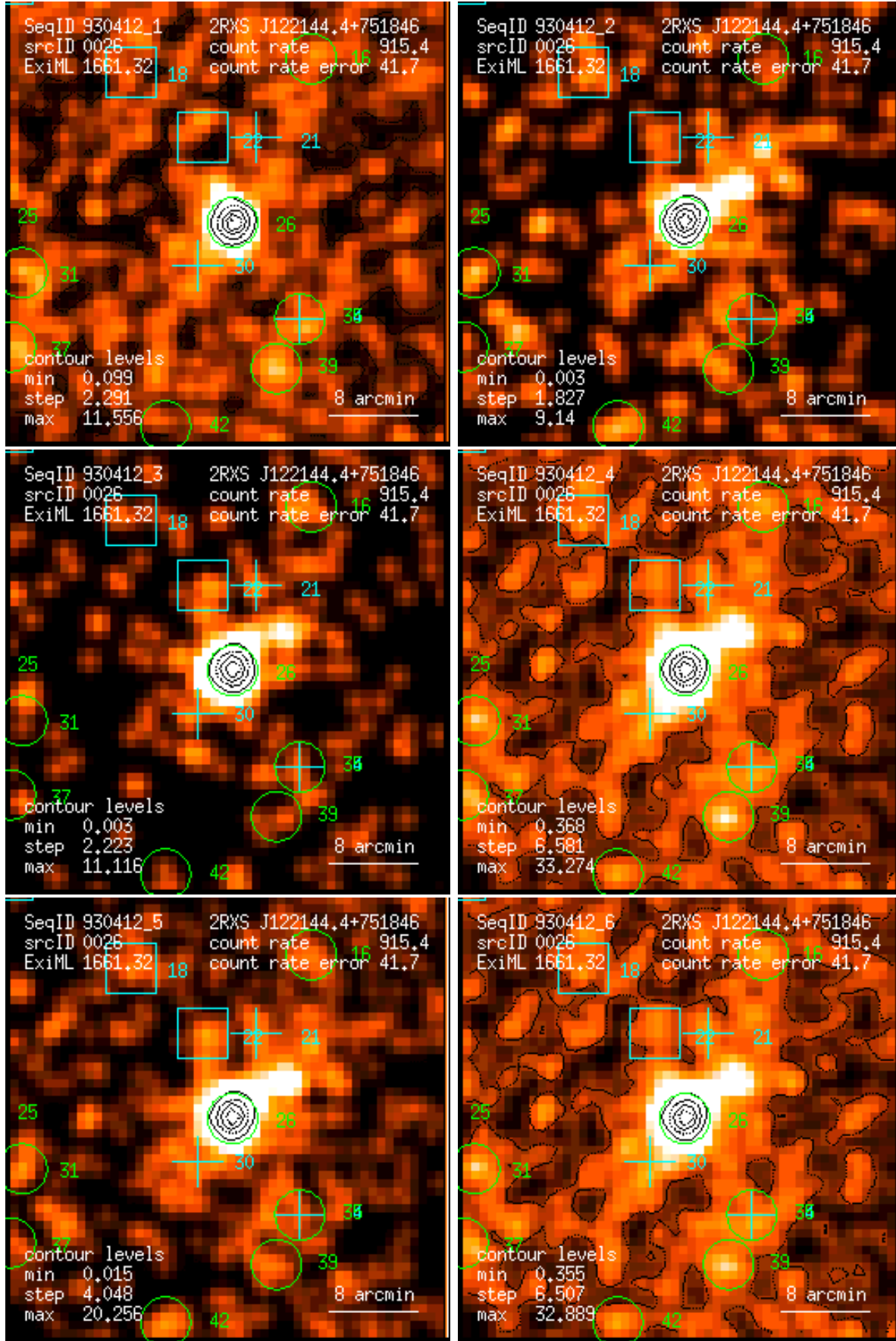
Figure 26: RASS 930412: detection 0026: band rate images, Gaussian filter: (1) PSPC channels 11 – 41, (2) 52 – 90, (3) 91 – 201, (4) 11 – 235, (5) 52 – 201, (6) 11 – 201. Broad band rates in counts/ks. Band rate contour levels in counts/ks/arcmin 2 .
