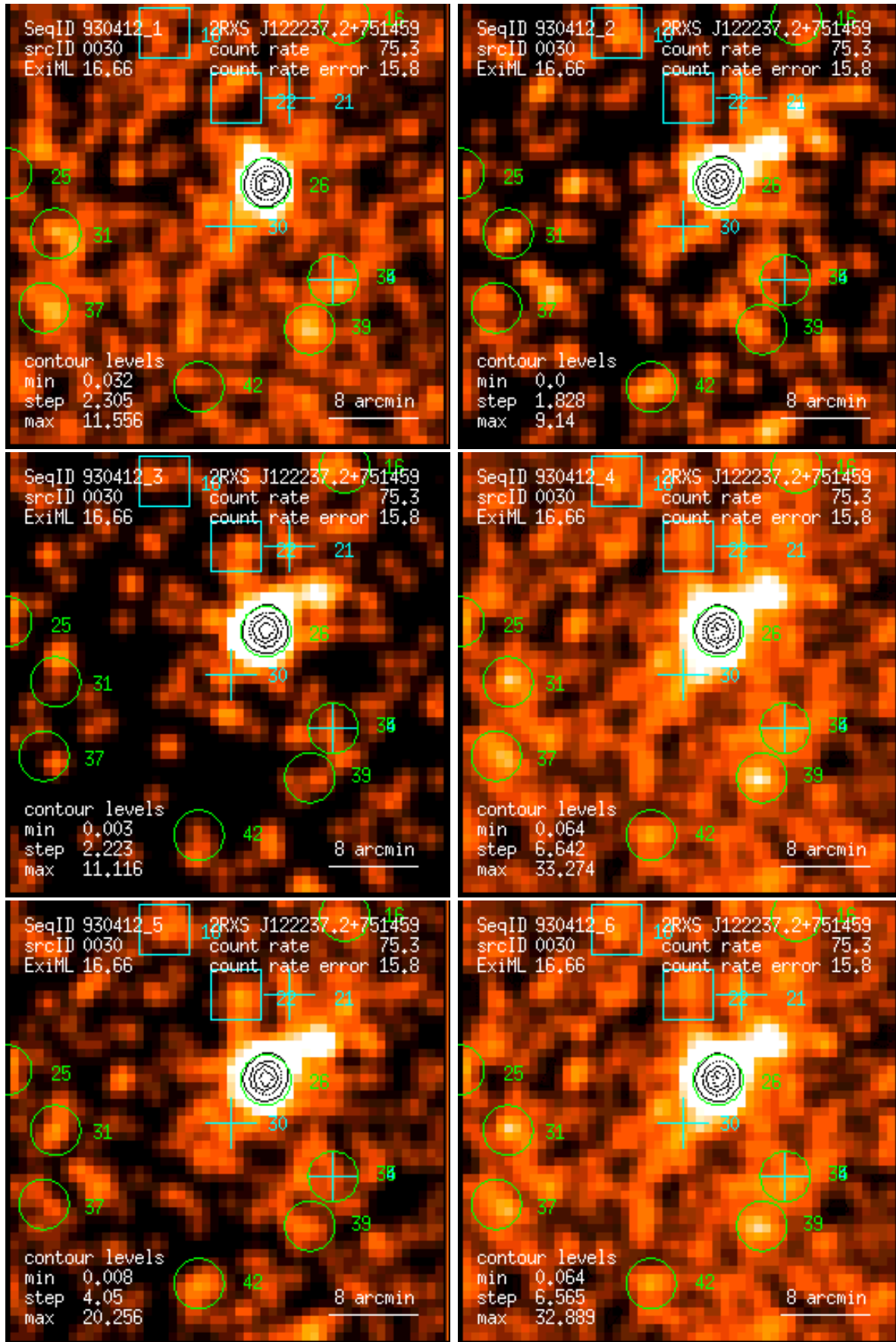
Figure 30: RASS 930412: detection 0030: band rate images, Gaussian filter: (1) PSPC channels 11 – 41, (2) 52 – 90, (3) 91 – 201, (4) 11 – 235, (5) 52 – 201, (6) 11 – 201. Broad band rates in counts/ks. Band rate contour levels in counts/ks/arcmin 2 .
