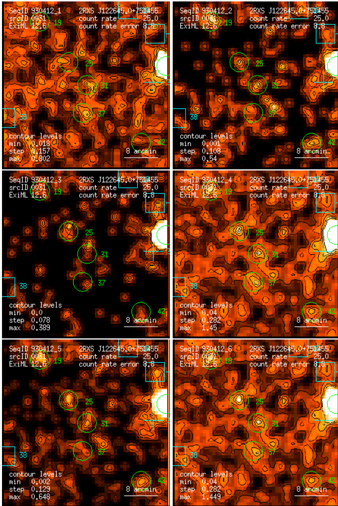
Figure 31: RASS 930412: detection 0031: band rate images, Gaussian filter: (1) PSPC channels 11 – 41, (2) 52 – 90, (3) 91 – 201, (4) 11 – 235, (5) 52 – 201, (6) 11 – 201. Broad band rates in counts/ks. Band rate contour levels in counts/ks/arcmin 2 .
