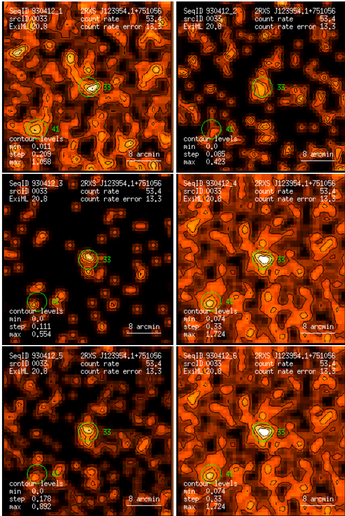
Figure 33: RASS 930412: detection 0033: band rate images, Gaussian filter: (1) PSPC channels 11 – 41, (2) 52 – 90, (3) 91 – 201, (4) 11 – 235, (5) 52 – 201, (6) 11 – 201. Broad band rates in counts/ks. Band rate contour levels in counts/ks/arcmin 2 .
