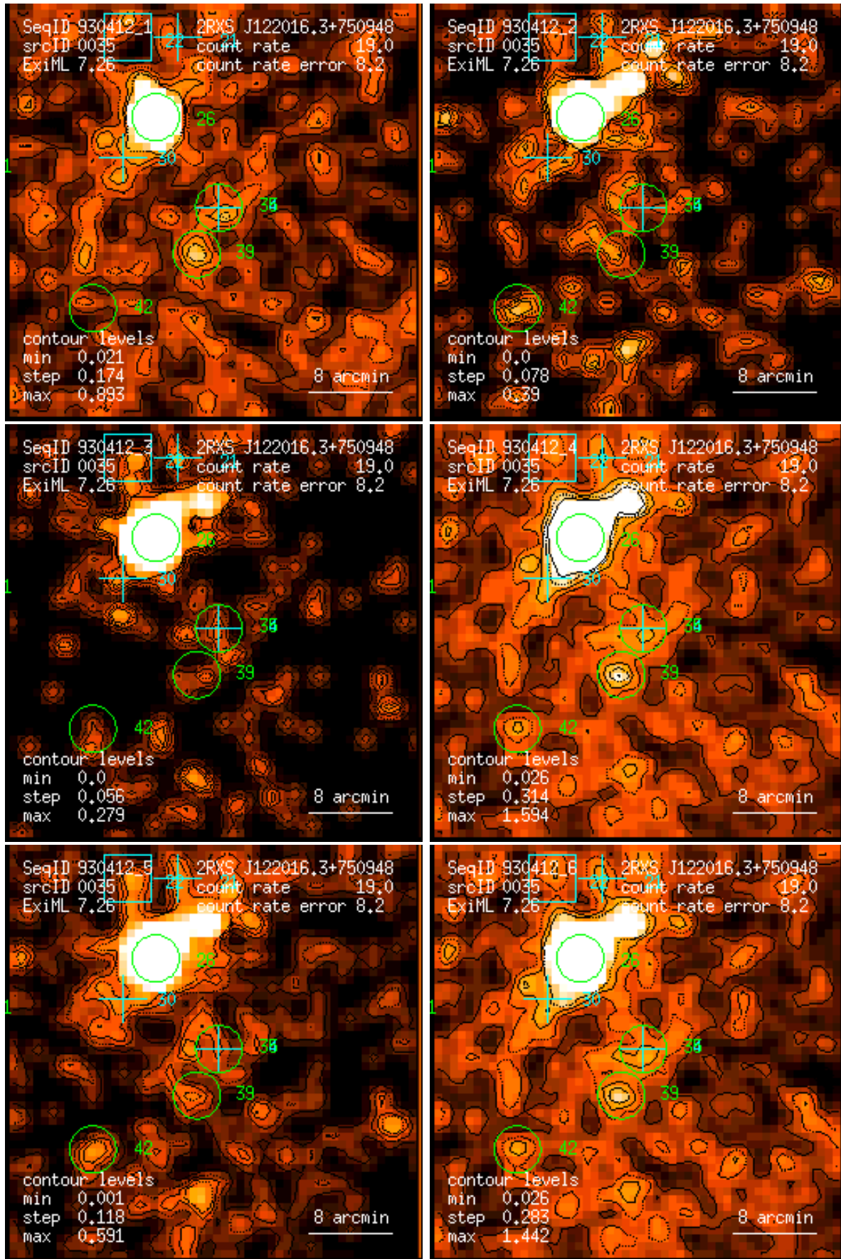
Figure 35: RASS 930412: detection 0035: band rate images, Gaussian filter: (1) PSPC channels 11 – 41, (2) 52 – 90, (3) 91 – 201, (4) 11 – 235, (5) 52 – 201, (6) 11 – 201. Broad band rates in counts/ks. Band rate contour levels in counts/ks/arcmin 2 .
