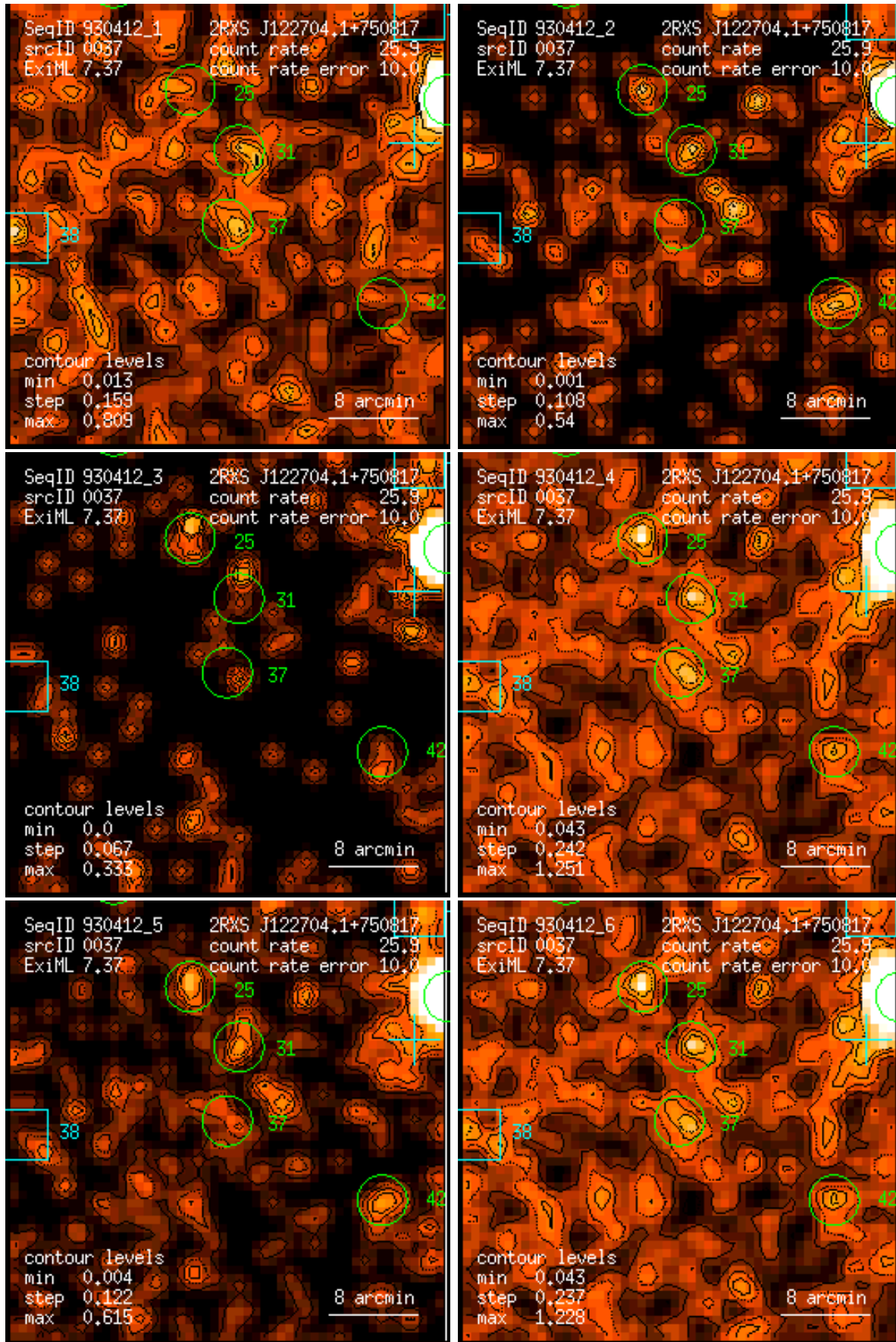
Figure 37: RASS 930412: detection 0037: band rate images, Gaussian filter: (1) PSPC channels 11 – 41, (2) 52 – 90, (3) 91 – 201, (4) 11 – 235, (5) 52 – 201, (6) 11 – 201. Broad band rates in counts/ks. Band rate contour levels in counts/ks/arcmin 2 .
