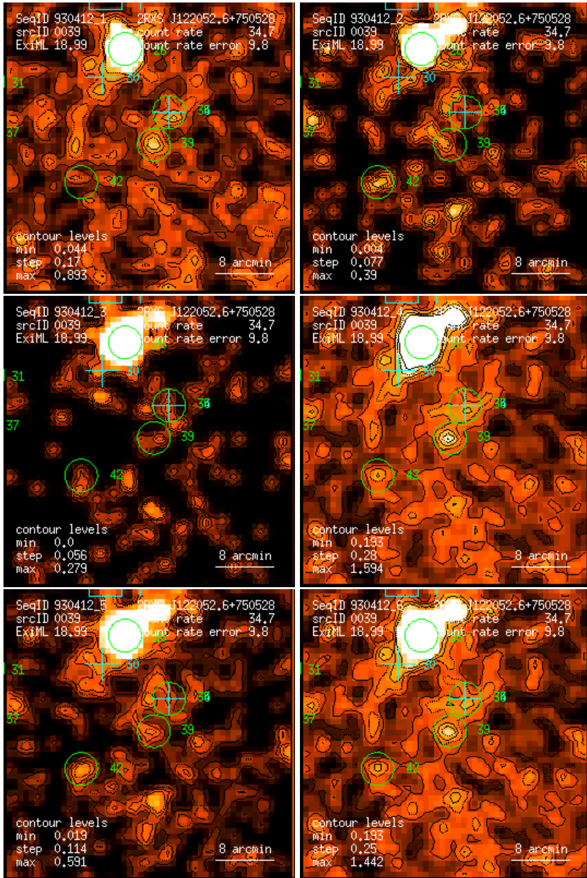
Figure 39: RASS 930412: detection 0039: band rate images, Gaussian filter: (1) PSPC channels 11 – 41, (2) 52 – 90, (3) 91 – 201, (4) 11 – 235, (5) 52 – 201, (6) 11 – 201. Broad band rates in counts/ks. Band rate contour levels in counts/ks/arcmin 2 .
