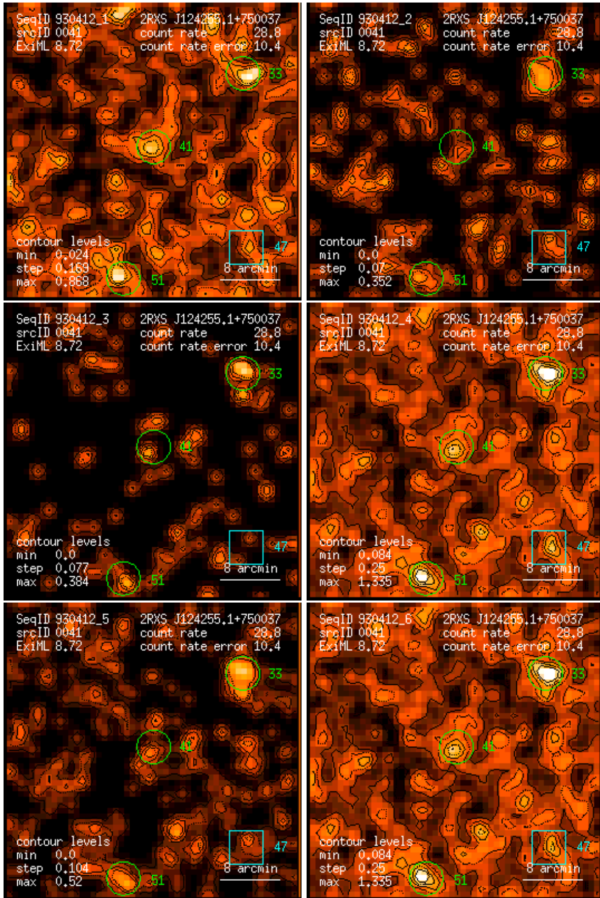
Figure 41: RASS 930412: detection 0041: band rate images, Gaussian filter: (1) PSPC channels 11 – 41, (2) 52 – 90, (3) 91 – 201, (4) 11 – 235, (5) 52 – 201, (6) 11 – 201. Broad band rates in counts/ks. Band rate contour levels in counts/ks/arcmin 2 .
