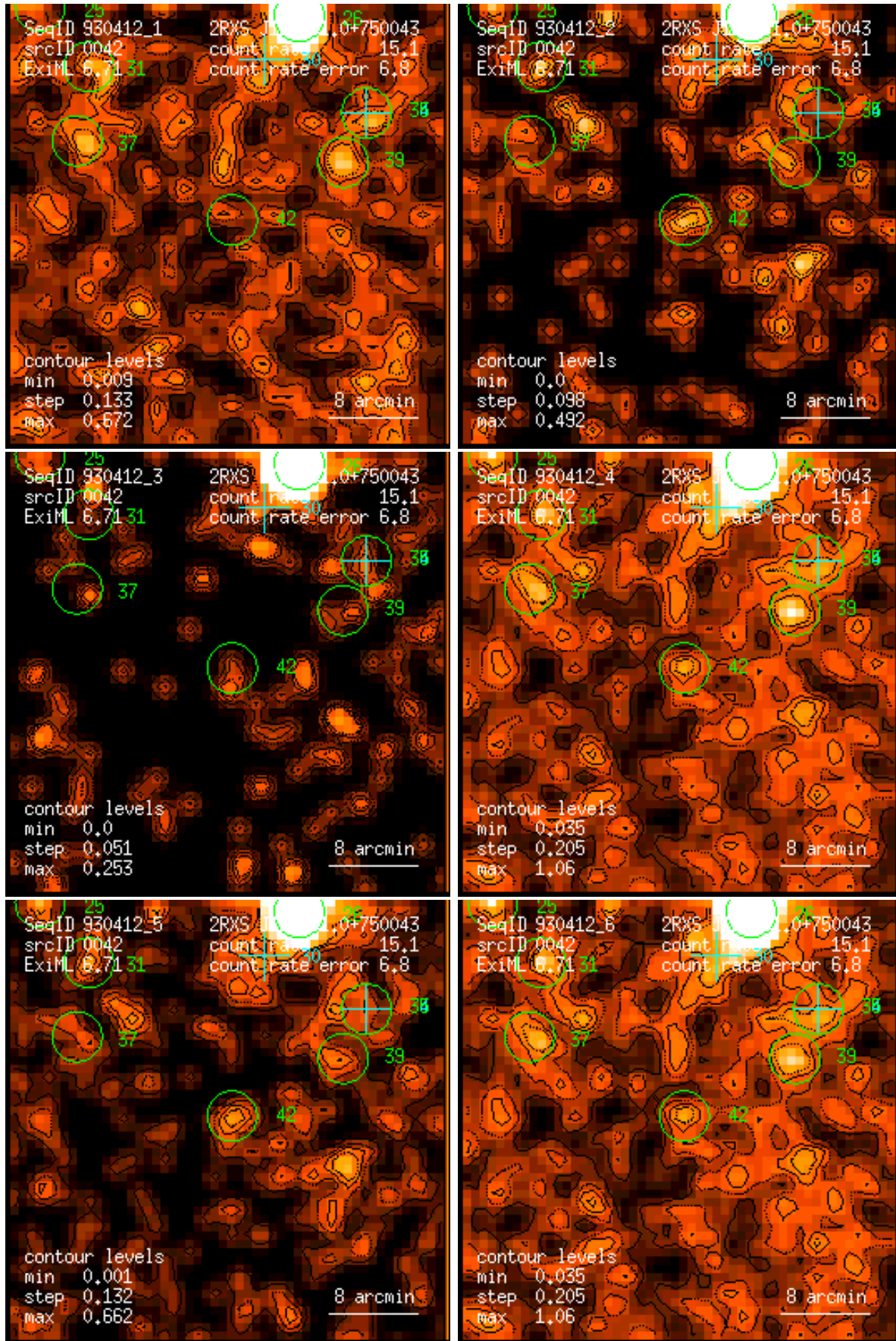
Figure 42: RASS 930412: detection 0042: band rate images, Gaussian filter: (1) PSPC channels 11 – 41, (2) 52 – 90, (3) 91 – 201, (4) 11 – 235, (5) 52 – 201, (6) 11 – 201. Broad band rates in counts/ks. Band rate contour levels in counts/ks/arcmin 2 .
