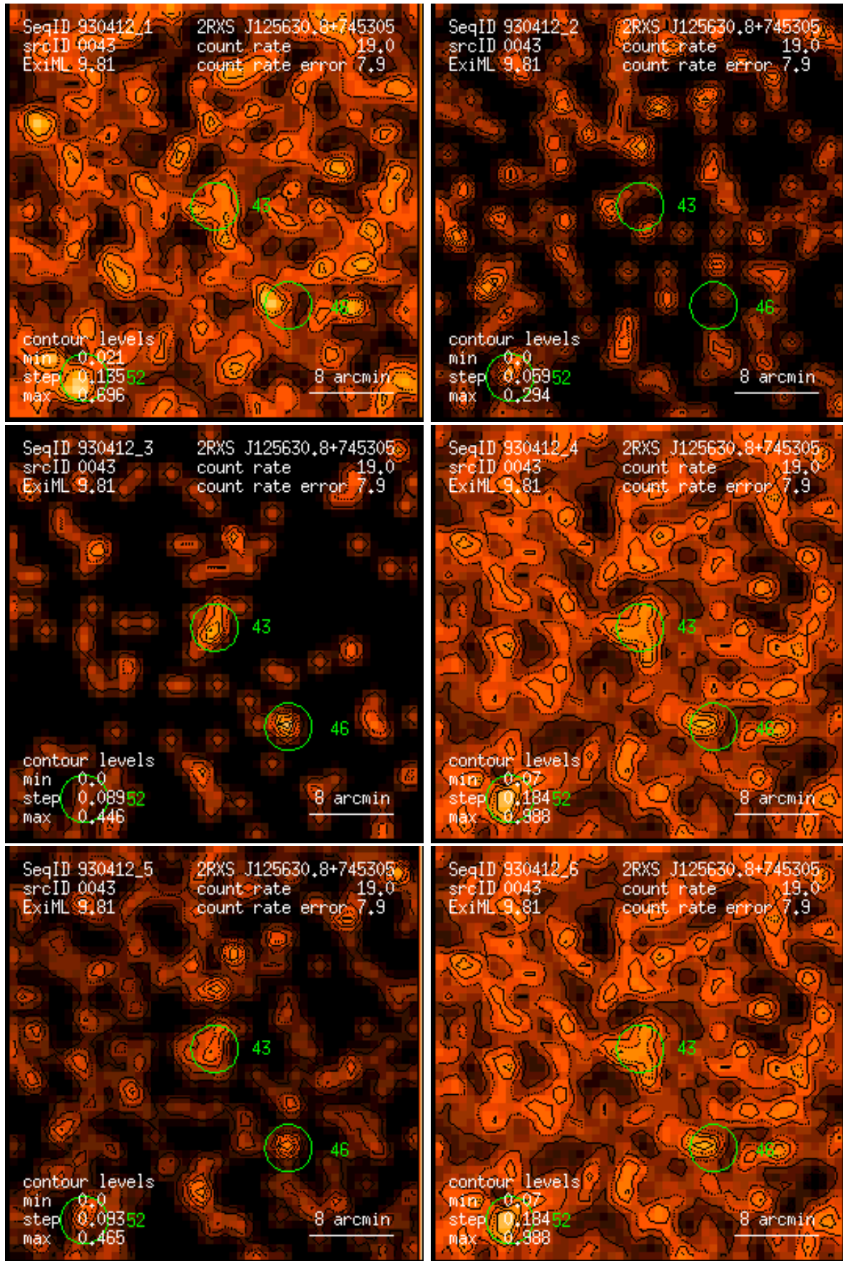
Figure 43: RASS 930412: detection 0043: band rate images, Gaussian filter: (1) PSPC channels 11 – 41, (2) 52 – 90, (3) 91 – 201, (4) 11 – 235, (5) 52 – 201, (6) 11 – 201. Broad band rates in counts/ks. Band rate contour levels in counts/ks/arcmin 2 .
