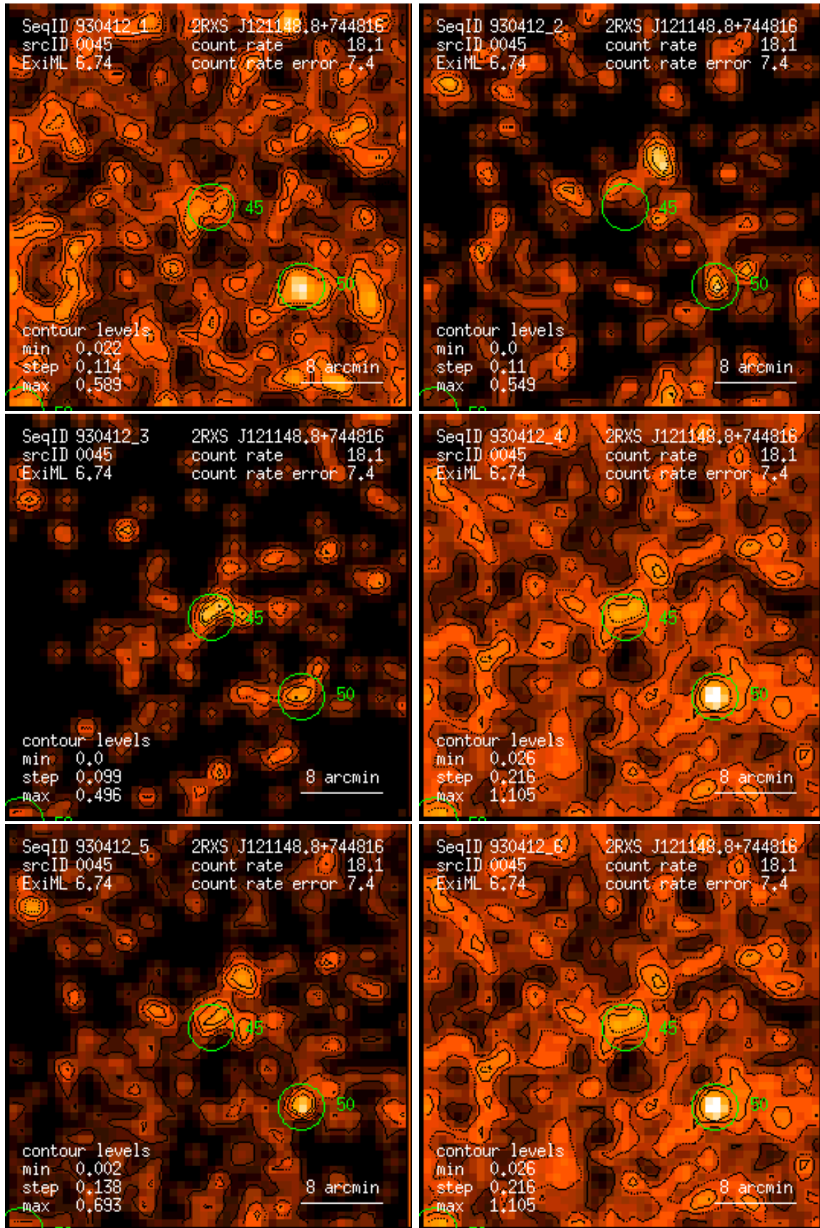
Figure 45: RASS 930412: detection 0045: band rate images, Gaussian filter: (1) PSPC channels 11 – 41, (2) 52 – 90, (3) 91 – 201, (4) 11 – 235, (5) 52 – 201, (6) 11 – 201. Broad band rates in counts/ks. Band rate contour levels in counts/ks/arcmin 2 .
