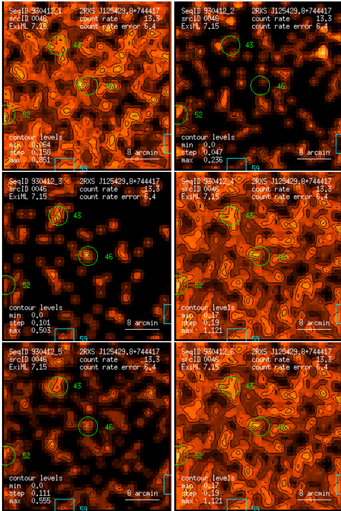
Figure 46: RASS 930412: detection 0046: band rate images, Gaussian filter: (1) PSPC channels 11 – 41, (2) 52 – 90, (3) 91 – 201, (4) 11 – 235, (5) 52 – 201, (6) 11 – 201. Broad band rates in counts/ks. Band rate contour levels in counts/ks/arcmin 2 .
