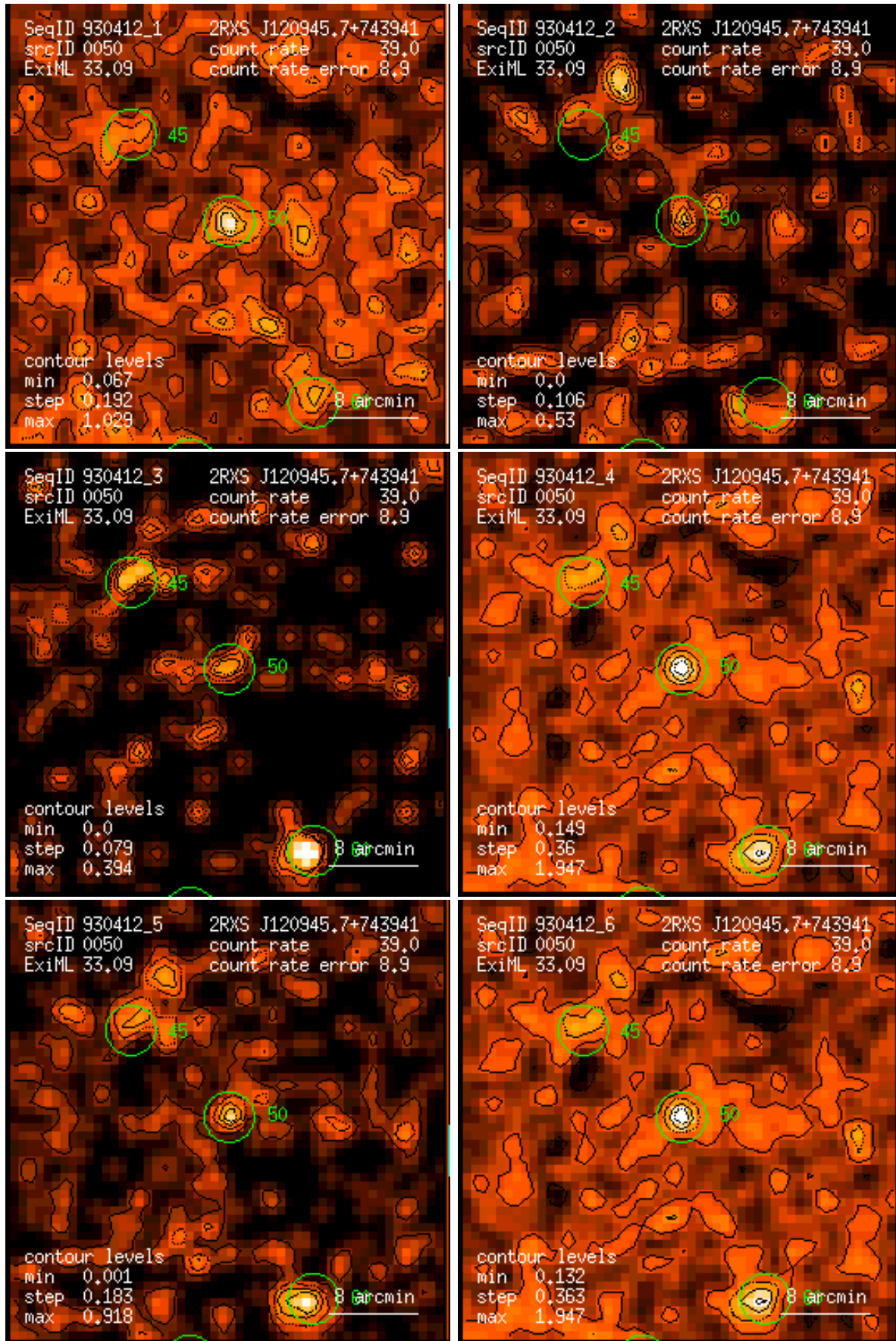
Figure 50: RASS 930412: detection 0050: band rate images, Gaussian filter: (1) PSPC channels 11 – 41, (2) 52 – 90, (3) 91 – 201, (4) 11 – 235, (5) 52 – 201, (6) 11 – 201. Broad band rates in counts/ks. Band rate contour levels in counts/ks/arcmin 2 .
