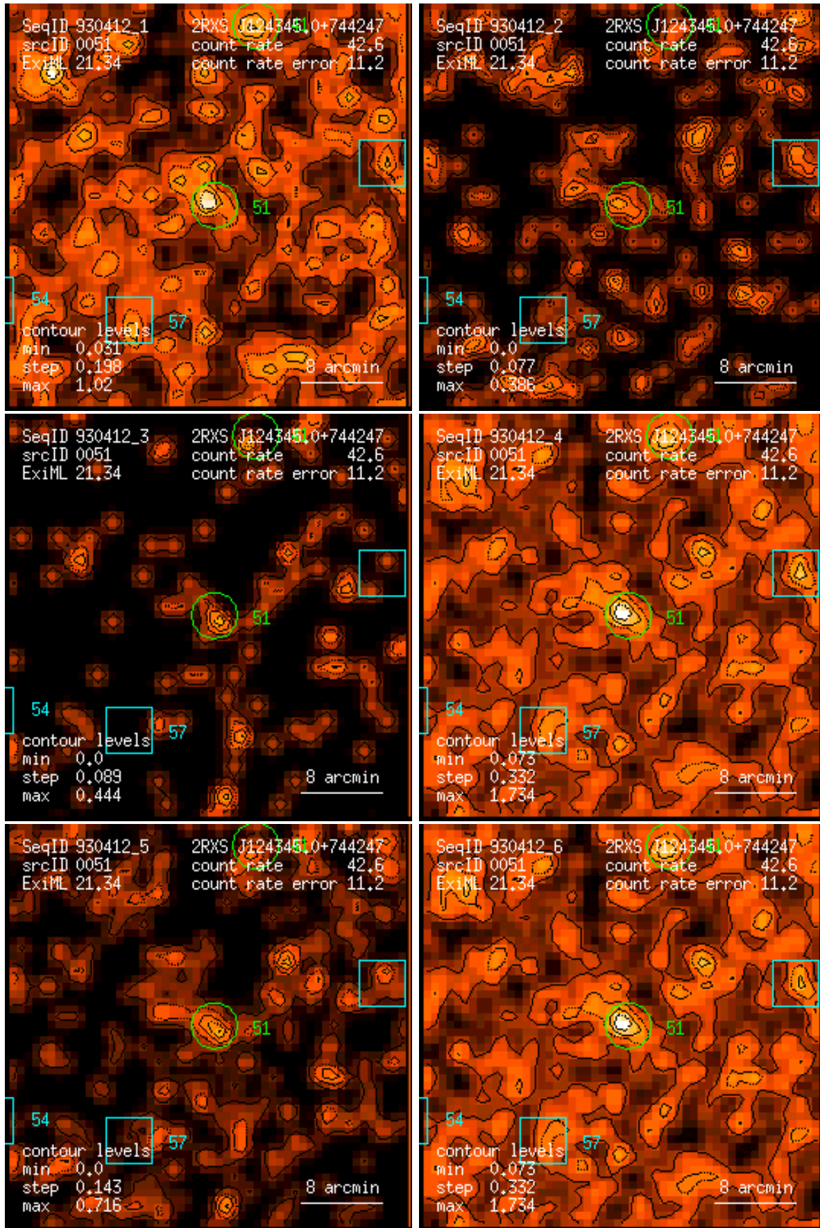
Figure 51: RASS 930412: detection 0051: band rate images, Gaussian filter: (1) PSPC channels 11 – 41, (2) 52 – 90, (3) 91 – 201, (4) 11 – 235, (5) 52 – 201, (6) 11 – 201. Broad band rates in counts/ks. Band rate contour levels in counts/ks/arcmin 2 .
