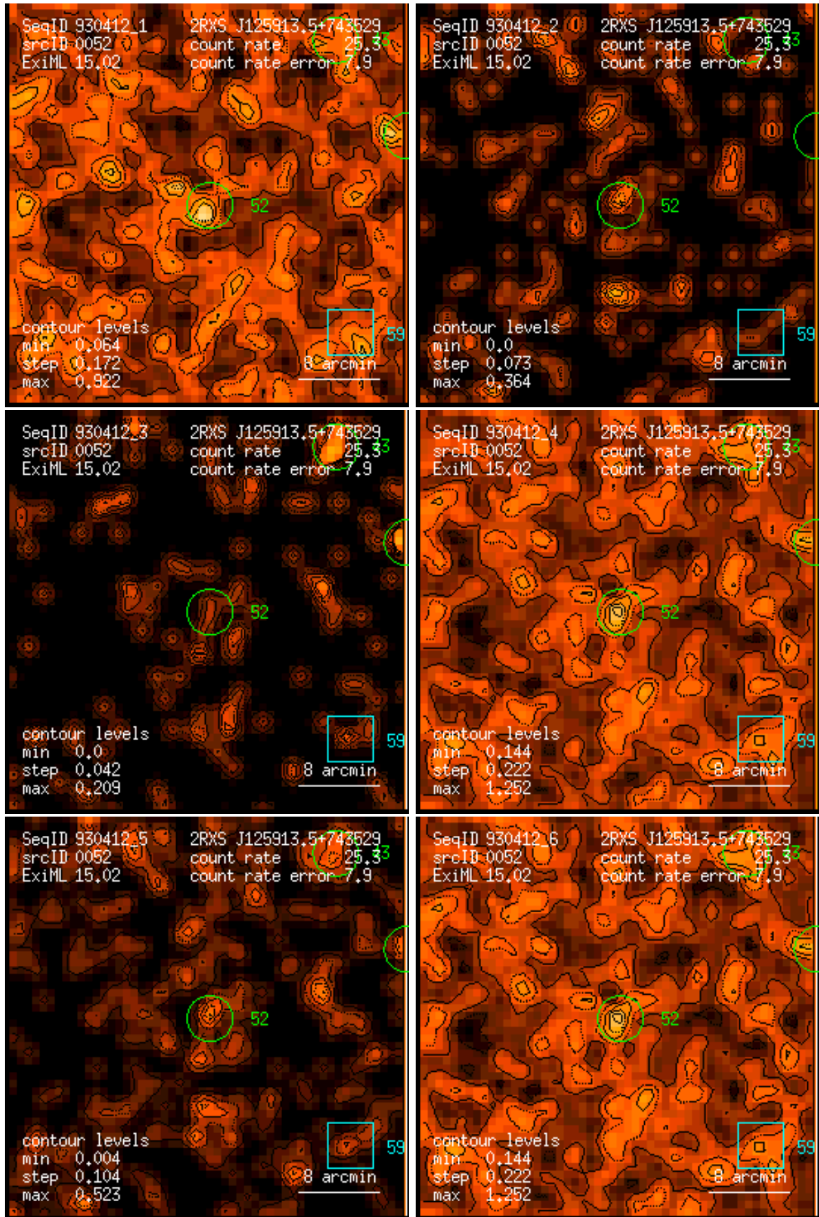
Figure 52: RASS 930412: detection 0052: band rate images, Gaussian filter: (1) PSPC channels 11 – 41, (2) 52 – 90, (3) 91 – 201, (4) 11 – 235, (5) 52 – 201, (6) 11 – 201. Broad band rates in counts/ks. Band rate contour levels in counts/ks/arcmin 2 .
