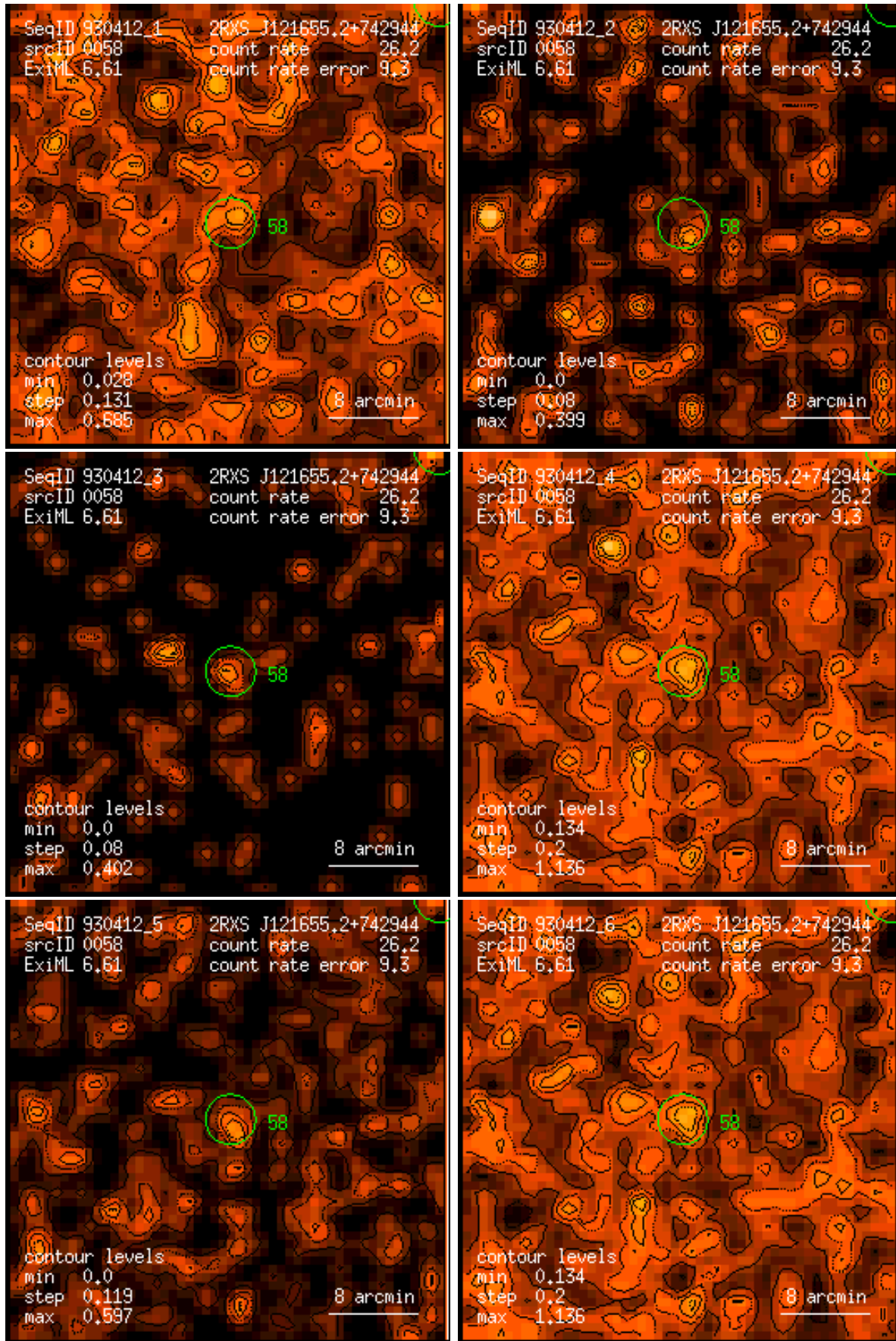
Figure 58: RASS 930412: detection 0058: band rate images, Gaussian filter: (1) PSPC channels 11 – 41, (2) 52 – 90, (3) 91 – 201, (4) 11 – 235, (5) 52 – 201, (6) 11 – 201. Broad band rates in counts/ks. Band rate contour levels in counts/ks/arcmin 2 .
