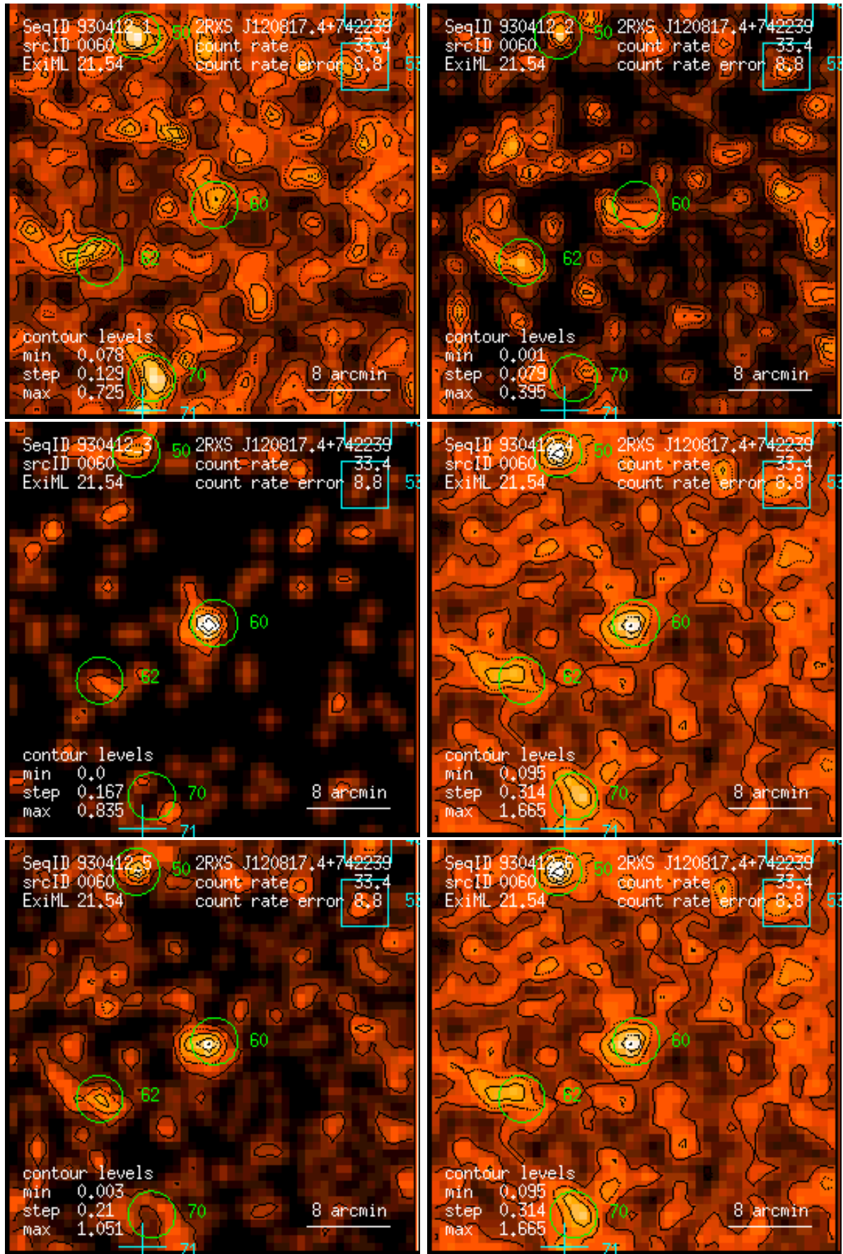
Figure 60: RASS 930412: detection 0060: band rate images, Gaussian filter: (1) PSPC channels 11 – 41, (2) 52 – 90, (3) 91 – 201, (4) 11 – 235, (5) 52 – 201, (6) 11 – 201. Broad band rates in counts/ks. Band rate contour levels in counts/ks/arcmin 2 .
