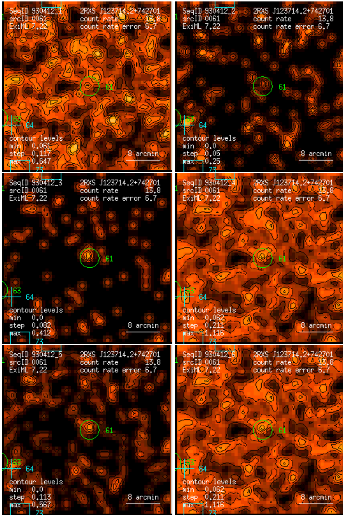
Figure 61: RASS 930412: detection 0061: band rate images, Gaussian filter: (1) PSPC channels 11 – 41, (2) 52 – 90, (3) 91 – 201, (4) 11 – 235, (5) 52 – 201, (6) 11 – 201. Broad band rates in counts/ks. Band rate contour levels in counts/ks/arcmin 2 .
