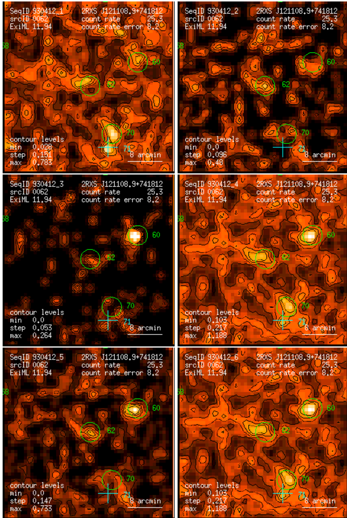
Figure 62: RASS 930412: detection 0062: band rate images, Gaussian filter: (1) PSPC channels 11 – 41, (2) 52 – 90, (3) 91 – 201, (4) 11 – 235, (5) 52 – 201, (6) 11 – 201. Broad band rates in counts/ks. Band rate contour levels in counts/ks/arcmin 2 .
