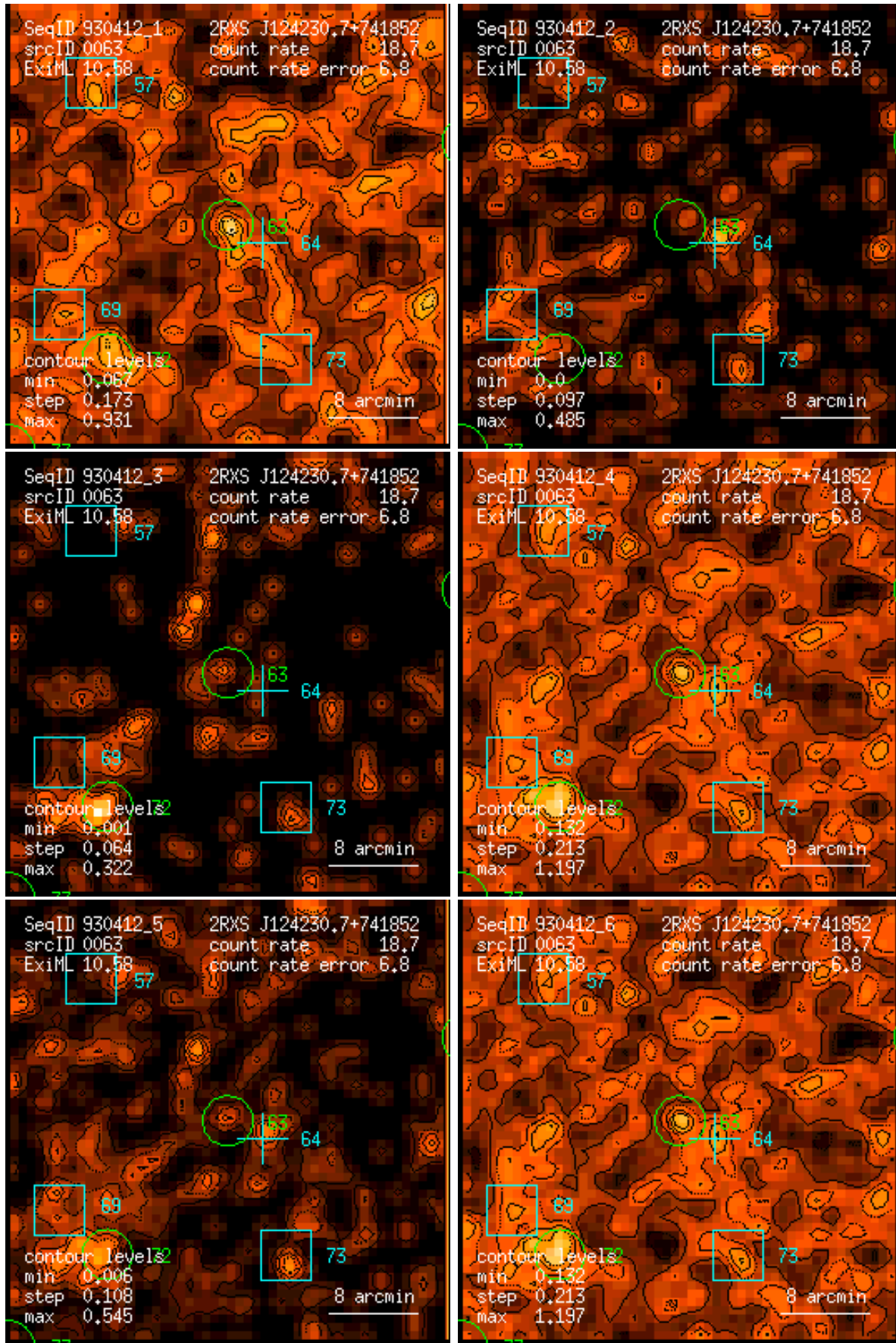
Figure 63: RASS 930412: detection 0063: band rate images, Gaussian filter: (1) PSPC channels 11 – 41, (2) 52 – 90, (3) 91 – 201, (4) 11 – 235, (5) 52 – 201, (6) 11 – 201. Broad band rates in counts/ks. Band rate contour levels in counts/ks/arcmin 2 .
