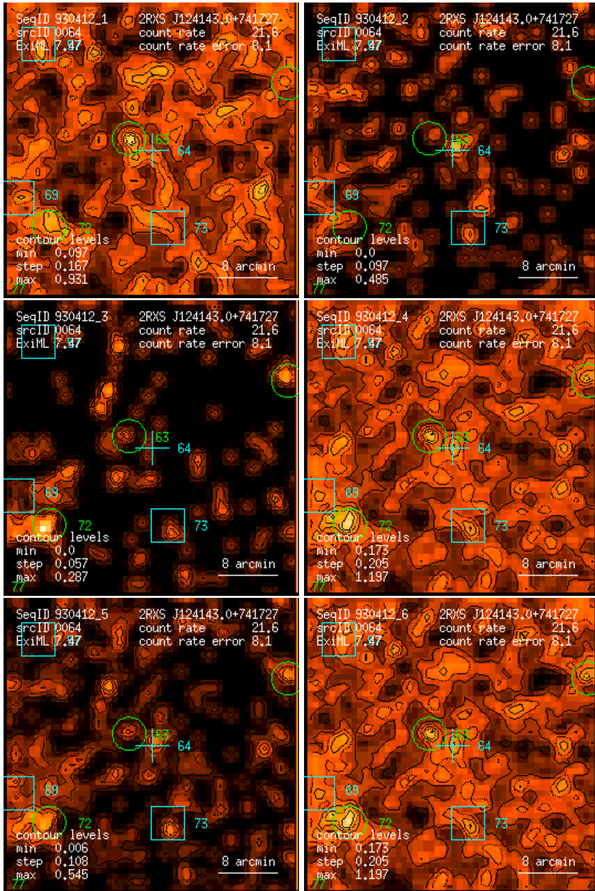
Figure 64: RASS 930412: detection 0064: band rate images, Gaussian filter: (1) PSPC channels 11 – 41, (2) 52 – 90, (3) 91 – 201, (4) 11 – 235, (5) 52 – 201, (6) 11 – 201. Broad band rates in counts/ks. Band rate contour levels in counts/ks/arcmin 2 .
