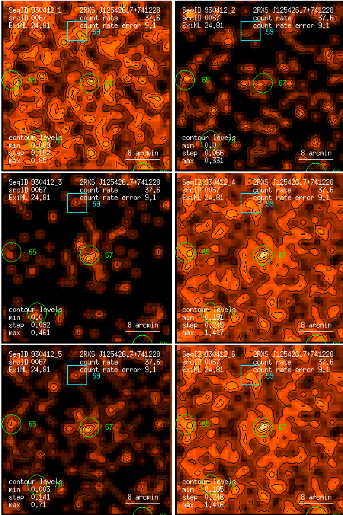
Figure 67: RASS 930412: detection 0067: band rate images, Gaussian filter: (1) PSPC channels 11 – 41, (2) 52 – 90, (3) 91 – 201, (4) 11 – 235, (5) 52 – 201, (6) 11 – 201. Broad band rates in counts/ks. Band rate contour levels in counts/ks/arcmin 2 .
