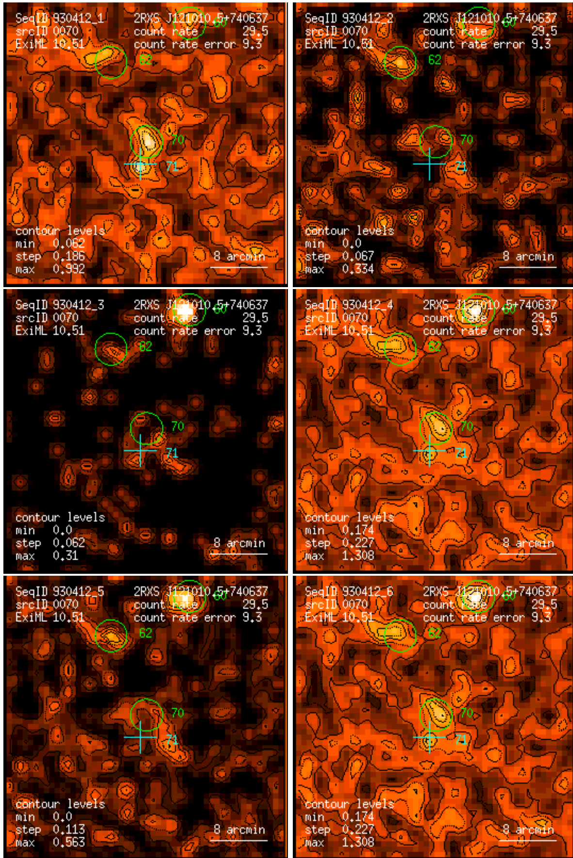
Figure 70: RASS 930412: detection 0070: band rate images, Gaussian filter: (1) PSPC channels 11 – 41, (2) 52 – 90, (3) 91 – 201, (4) 11 – 235, (5) 52 – 201, (6) 11 – 201. Broad band rates in counts/ks. Band rate contour levels in counts/ks/arcmin 2 .
