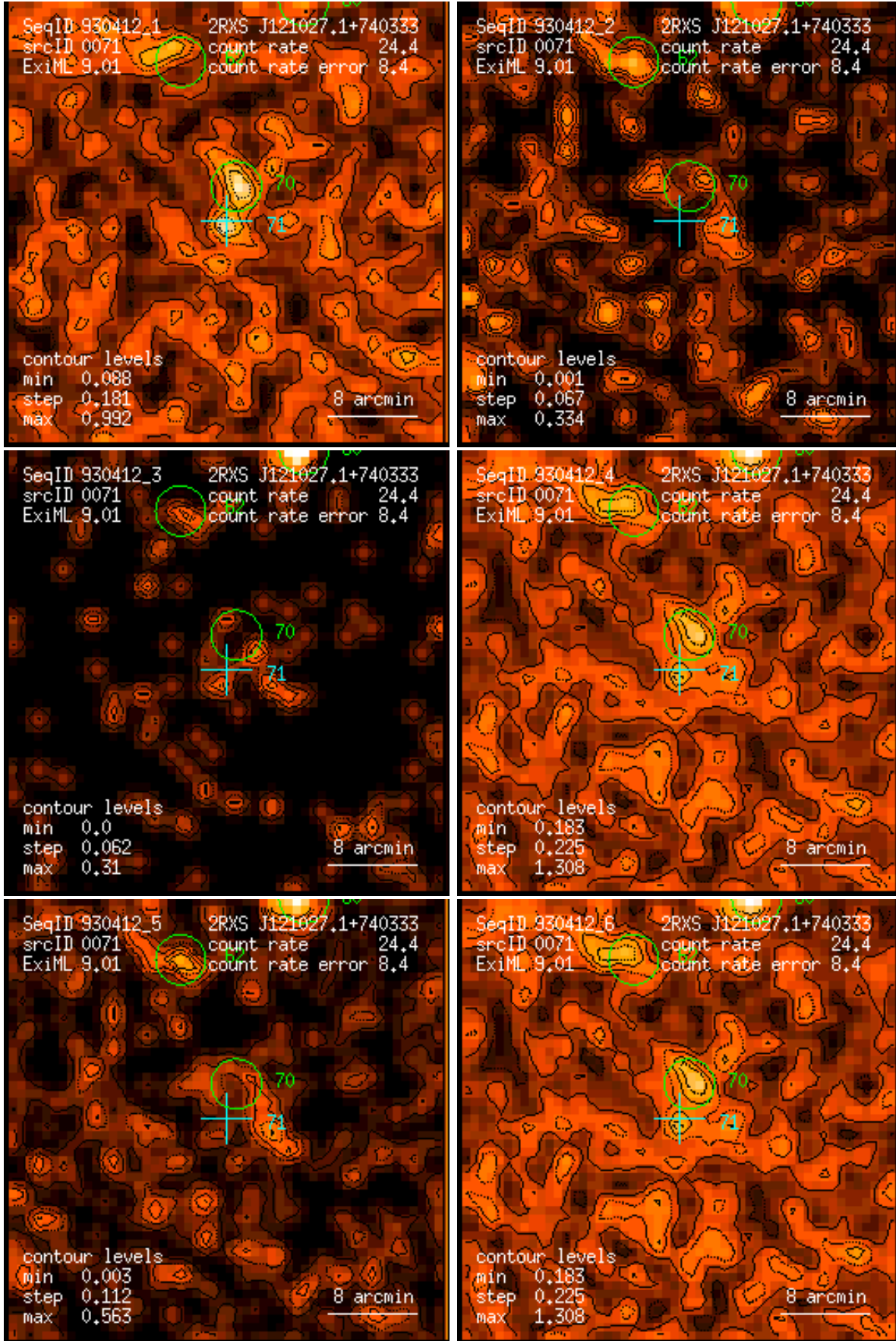
Figure 71: RASS 930412: detection 0071: band rate images, Gaussian filter: (1) PSPC channels 11 – 41, (2) 52 – 90, (3) 91 – 201, (4) 11 – 235, (5) 52 – 201, (6) 11 – 201. Broad band rates in counts/ks. Band rate contour levels in counts/ks/arcmin 2 .
