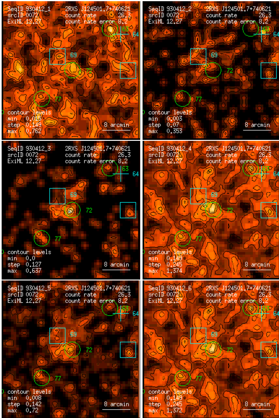
Figure 72: RASS 930412: detection 0072: band rate images, Gaussian filter: (1) PSPC channels 11 – 41, (2) 52 – 90, (3) 91 – 201, (4) 11 – 235, (5) 52 – 201, (6) 11 – 201. Broad band rates in counts/ks. Band rate contour levels in counts/ks/arcmin 2 .
