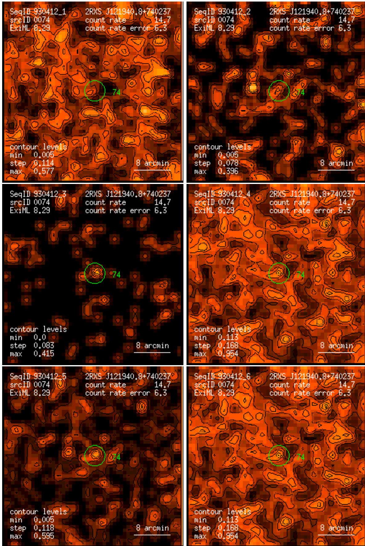
Figure 74: RASS 930412: detection 0074: band rate images, Gaussian filter: (1) PSPC channels 11 – 41, (2) 52 – 90, (3) 91 – 201, (4) 11 – 235, (5) 52 – 201, (6) 11 – 201. Broad band rates in counts/ks. Band rate contour levels in counts/ks/arcmin 2 .
