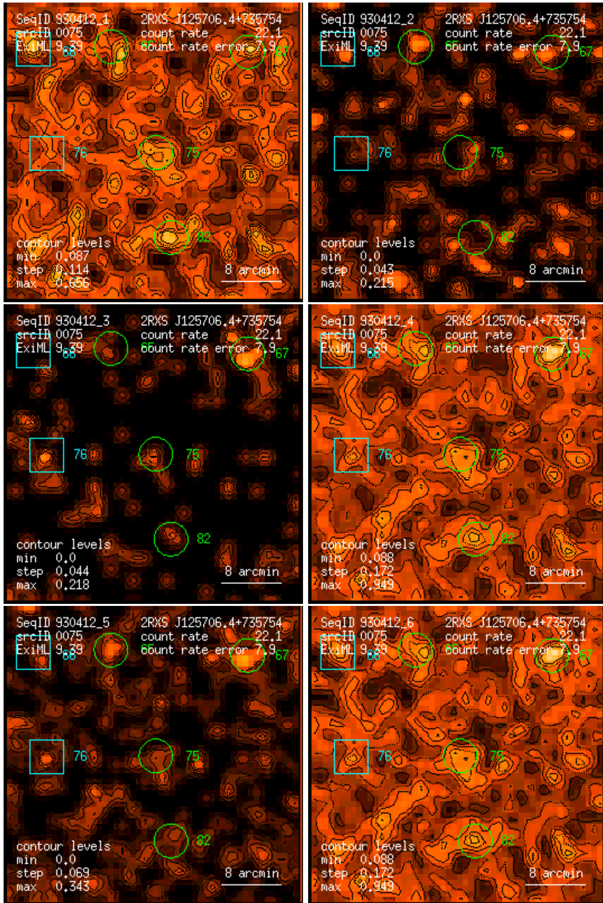
Figure 75: RASS 930412: detection 0075: band rate images, Gaussian filter: (1) PSPC channels 11 – 41, (2) 52 – 90, (3) 91 – 201, (4) 11 – 235, (5) 52 – 201, (6) 11 – 201. Broad band rates in counts/ks. Band rate contour levels in counts/ks/arcmin 2 .
