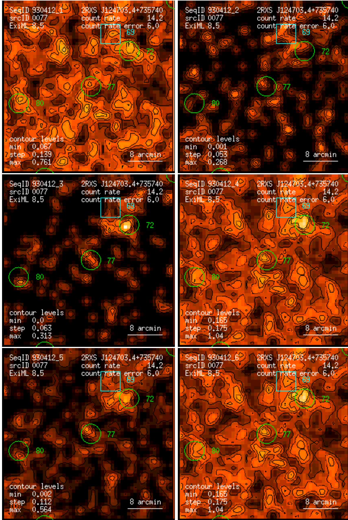
Figure 77: RASS 930412: detection 0077: band rate images, Gaussian filter: (1) PSPC channels 11 – 41, (2) 52 – 90, (3) 91 – 201, (4) 11 – 235, (5) 52 – 201, (6) 11 – 201. Broad band rates in counts/ks. Band rate contour levels in counts/ks/arcmin 2 .
