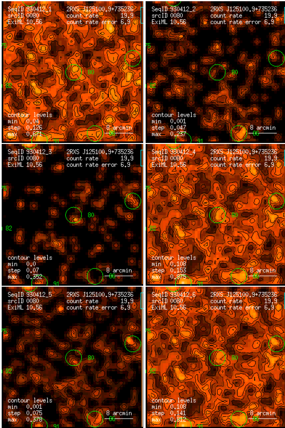
Figure 80: RASS 930412: detection 0080: band rate images, Gaussian filter: (1) PSPC channels 11 – 41, (2) 52 – 90, (3) 91 – 201, (4) 11 – 235, (5) 52 – 201, (6) 11 – 201. Broad band rates in counts/ks. Band rate contour levels in counts/ks/arcmin 2 .
